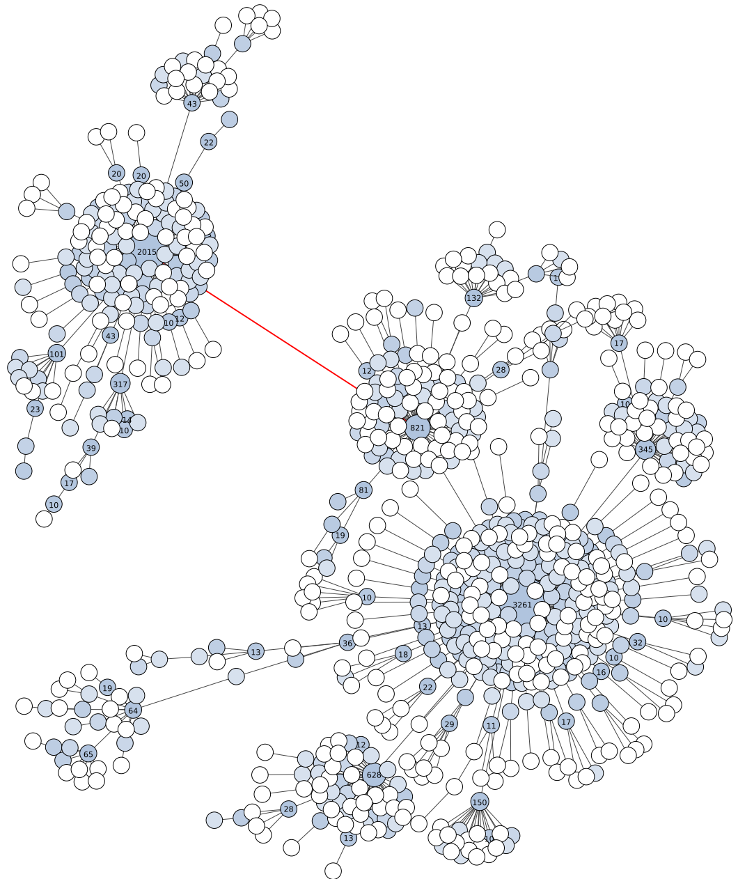
Figure 2 Graphical representation of an OTU produced by Swarm (breaking and grafting phases deactivated) when clustering the BioMarKs 18S rRNA V9 dataset (amplicons are appr. 129 bp in length). Nodes represent amplicons. Node size, color and text annotations represent the abundance of each amplicon. Edges represent one difference (substitution, deletion or insertion); the length of the edges carries no information. The red-colored edge indicates where Swarm's breaking phase cuts when it is not deactivated, resulting into two high abundant OTUs, each being assigned to a different genus of Collodaria (Radiolaria).
