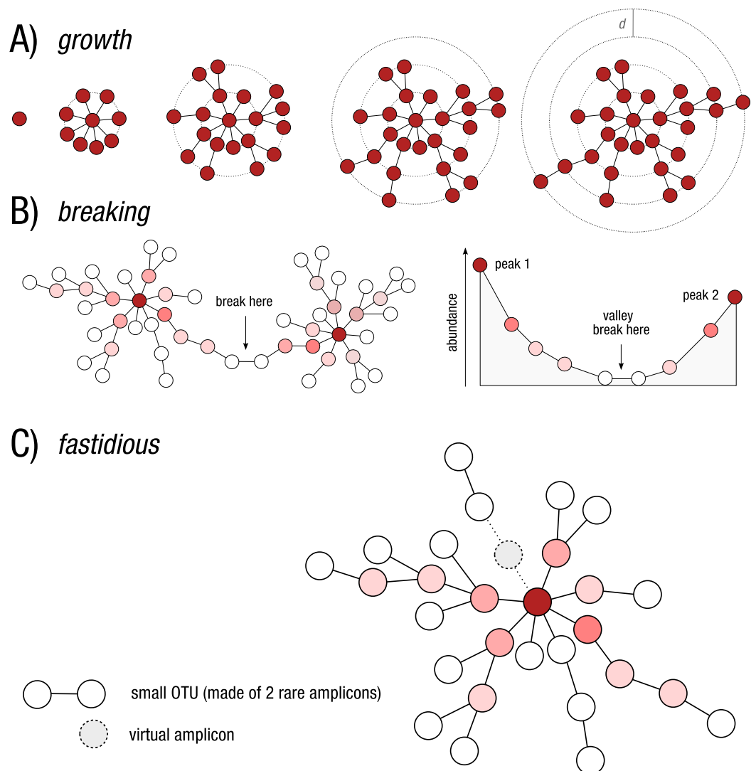
Figure 1 Schematic view of Swarm's clustering and refinement approach. (A) Swarm clusters amplicons iteratively by using a small user-chosen local threshold, d , allowing OTUs to grow to their natural limits, where no other amplicons can be added. (B) Swarm takes into account the abundance of each amplicon to produce higher resolution clusters, by not allowing the formation of amplicon chains. The darker the red, the higher the abundance. (C) The fastidious option avoids under-grouping (e.g., the production of small OTUs such as singletons and doubletons) by postulating the existence of virtual linking amplicons to graft smaller OTUs onto larger ones.
