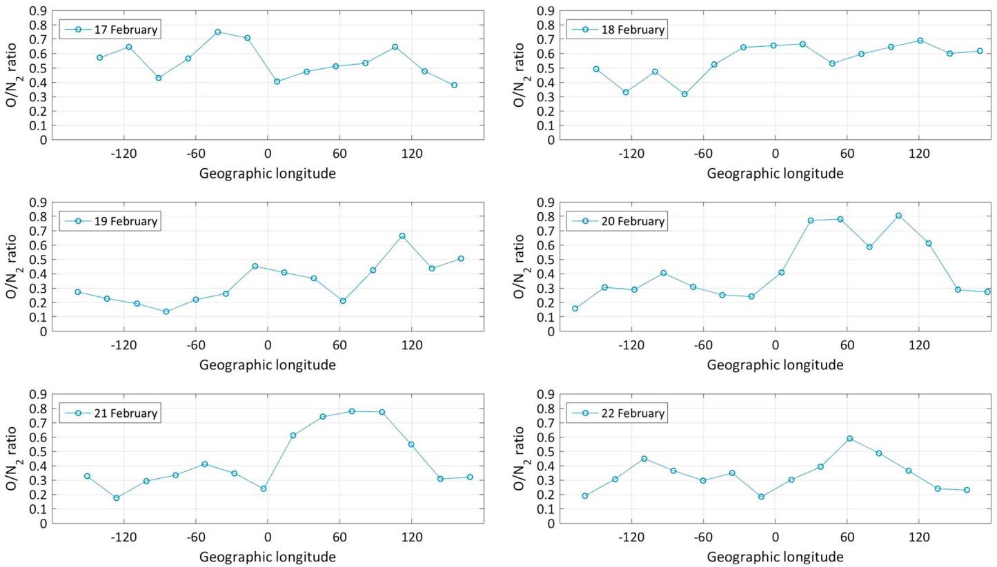
Figure 6. Longitudinal profiles demonstrating O/N 2 ratios (unitless) along 73° north latitude. The first CME hit on 19 February and the second on 20 February.
