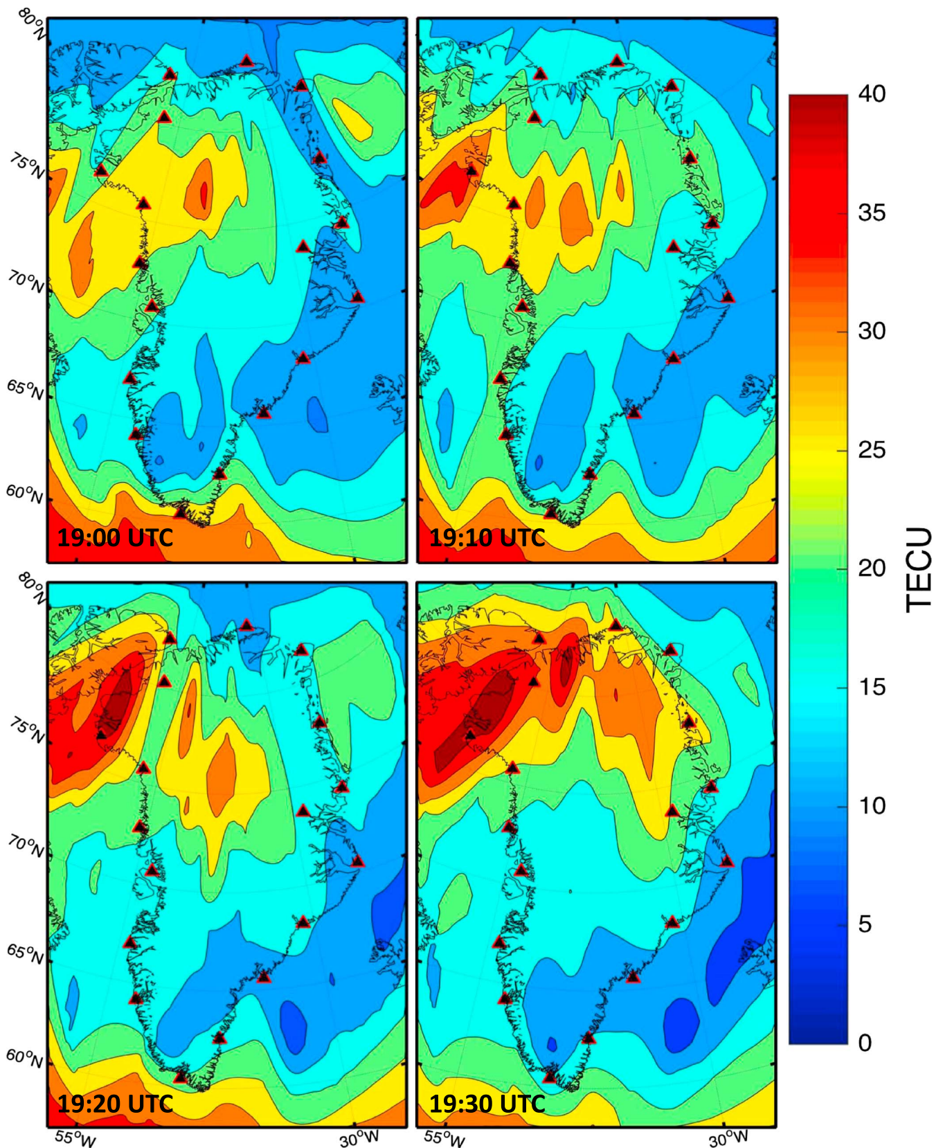
Figure 8. Polar patch structure progression over time shown from 19:00 to 19:30 UTC on 18 February 2014. The panels represent 10 min increments. The negative TEC anomaly along 65° latitude lies between the polar cap convection zones and the midlatitude ionosphere.
