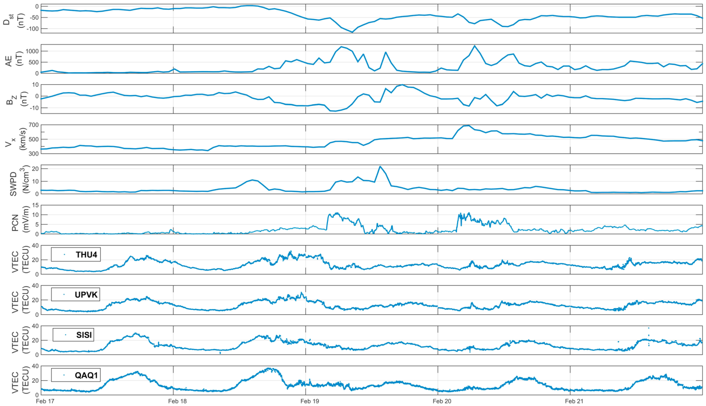
Figure 2. Near-Earth solar wind, interplanetary magnetic field (IMF), and plasma parameters shown in addition to the computed MVTEC using four Greenlandic GNSS stations on 17–21 February 2014: (first panel) Dst index, (second panel) AE index, (third panel) IMF B_z component, (fourth panel) Operating Missions as Nodes on the Internet (OMNI) solar wind velocity x component, (fifth panel) OMNI solar wind proton density, (sixth panel) PC north index, and (seventh to tenth panels) MVTEC values in order of decreasing station geographic latitude: Thule (77°28′00″N, 69°13′50″W), Upernavik (72°47′13″N, 56°08′50″W), Sisimiut (66°56′20″N, 53°40′20″W), and Qaortoq (60°43′20″N, 46°02′24″W). The red dashed lines mark the approximate times when the first (A) and second (B) CME-induced effects were detected in the observations.
