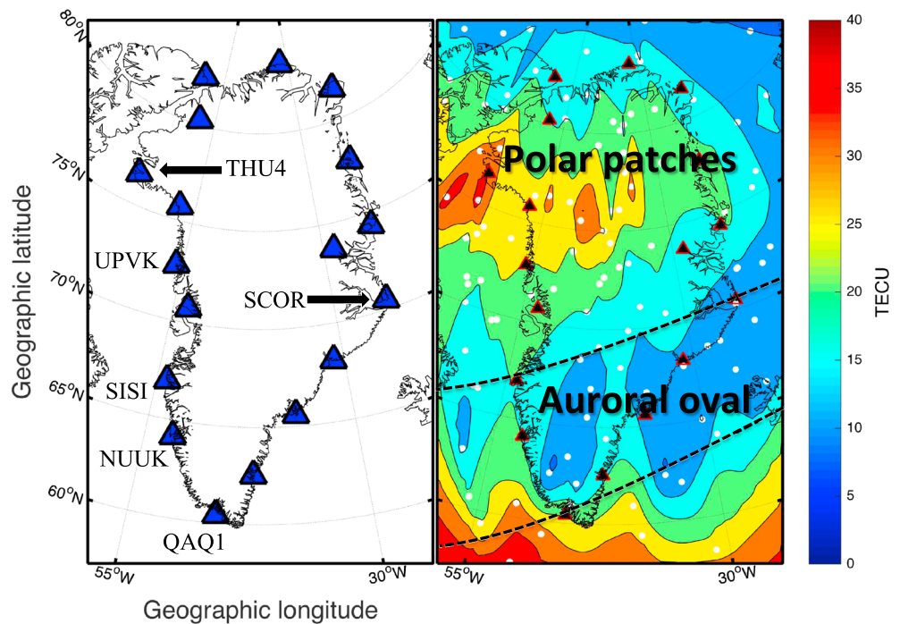
Figure 1. (left) Map of Greenland with blue triangles marking the locations of a subset of GNET GNSS stations that has been used to generate the VTEC maps in this study. Six out of the 18 stations were specifically labeled so their locations will be easily identified in later figures. Legend for the station codes are as follows: Nuuk (NUUK), Qaqortoq (QAQ1), Scorebysund (SCOR), Sisimiut (SISI), Thule (THU4), and Upernavik (UPVK). Note that the Thule ionosonde station is collocated with the Thule GNSS station for all practical purposes. (right) An example for VTEC map over Greenland at 19:15:00 (UTC), 18 February 2014, the day before the CME impact. The VTEC values at the ionospheric pierce points are denoted with white circles. The mapping was performed by employing the commonly used natural neighbor interpolation scheme to estimate values using the IPP values. The map clearly demonstrates local ionospheric structures [see, e.g., Rodger et al. , 1992] and polar patches. Due to the experimental setup auroral-E ionization (AEI) is not clearly apparent in this figure (for further details on AEI detection see Coker et al. [1995]). The auroral oval boundaries for this particular time are taken from The Johns Hopkins University Auroral Particles and Imagery website ( http://sd-www.jhuapl.edu/Aurora/ovation/ovation_display.html ).
