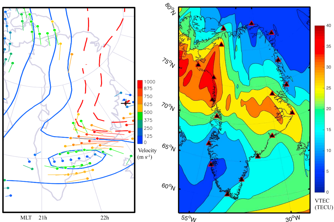
Figure 7. (left) SuperDARN drift velocities and contours of magnetospheric electric field potentials shown at 23:30 UTC on 18 February 2014 based on SuperDARN. The region between the two-cell convection pattern is located over Greenland (between red and blue potential contours). Antisunward convection of midlatitude-originated plasma is drifting over the polar cap there (when B_z points downward as shown in Figure 2). The closed blue contour surrounds a stagnation zone that results in increased plasma decay; compare this area with the same location on Figure 7 (right). (right) VTEC map covering the same geographical extent as Figure 7 (left). It was derived using 18 GNSS stations (black triangles with red edge) in Greenland. The interpolation is made from approximately 200 IPPs. The figure clearly shows connected but nonuniform patches near the intercell, antisunward convection zone.
