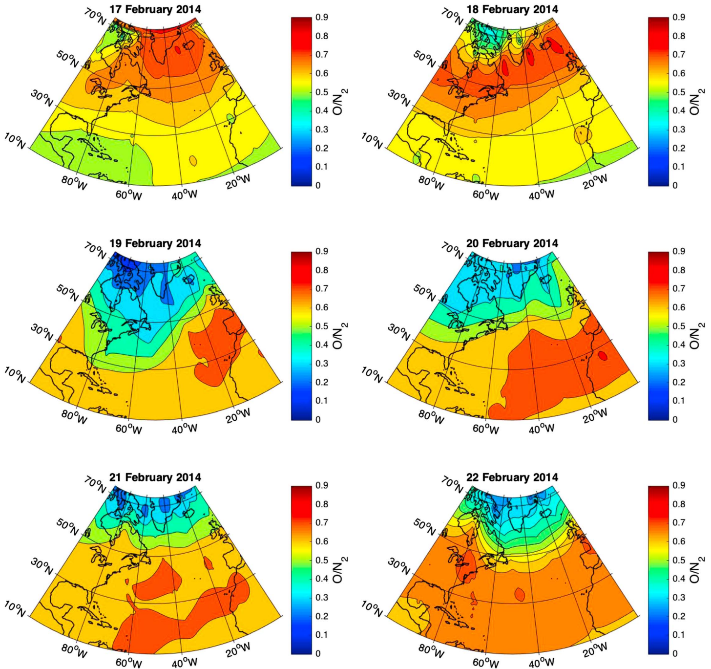
Figure 5. O/N_2 ratio maps demonstrating composition changes during the 6 days we investigated. The first CME hit on 19 February and the second on 20 February. The northernmost slice of these maps is shown in Figure 6.
