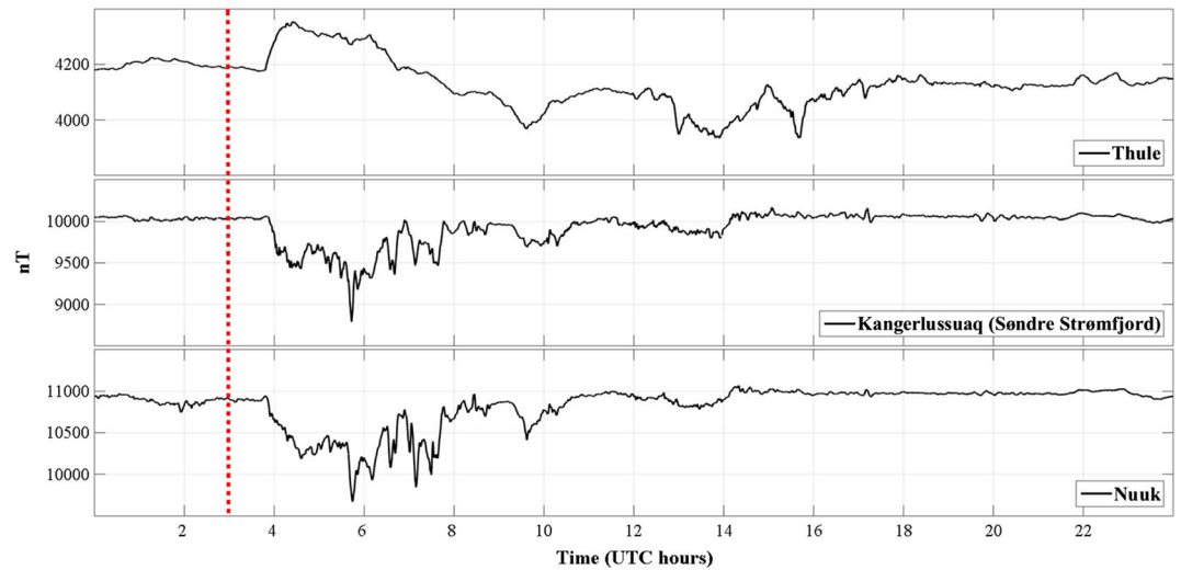
Figure 3. The 1 Hz vector variometer measurements from Greenlandic ground stations of the magnetic field vector north component on 19 February 2014. Thule is the northernmost and Nuuk is the southernmost station among the three indicated in the figure. The USGS National Geomagnetism website estimated that the first CME reached the Earth’s magnetopause around 03:00 UTC (marked by the vertical red dotted line). Among these three stations the Nuuk magnetic north component indicated the first changes, then ~10 s later they were observed at Kangerlussuaq, and finally ~100 s later they were observed at Thule. The timing accuracy of the instruments is \pm 2 s. The local ground magnetic response was delayed by almost 1 h compared to the Dst drop.
