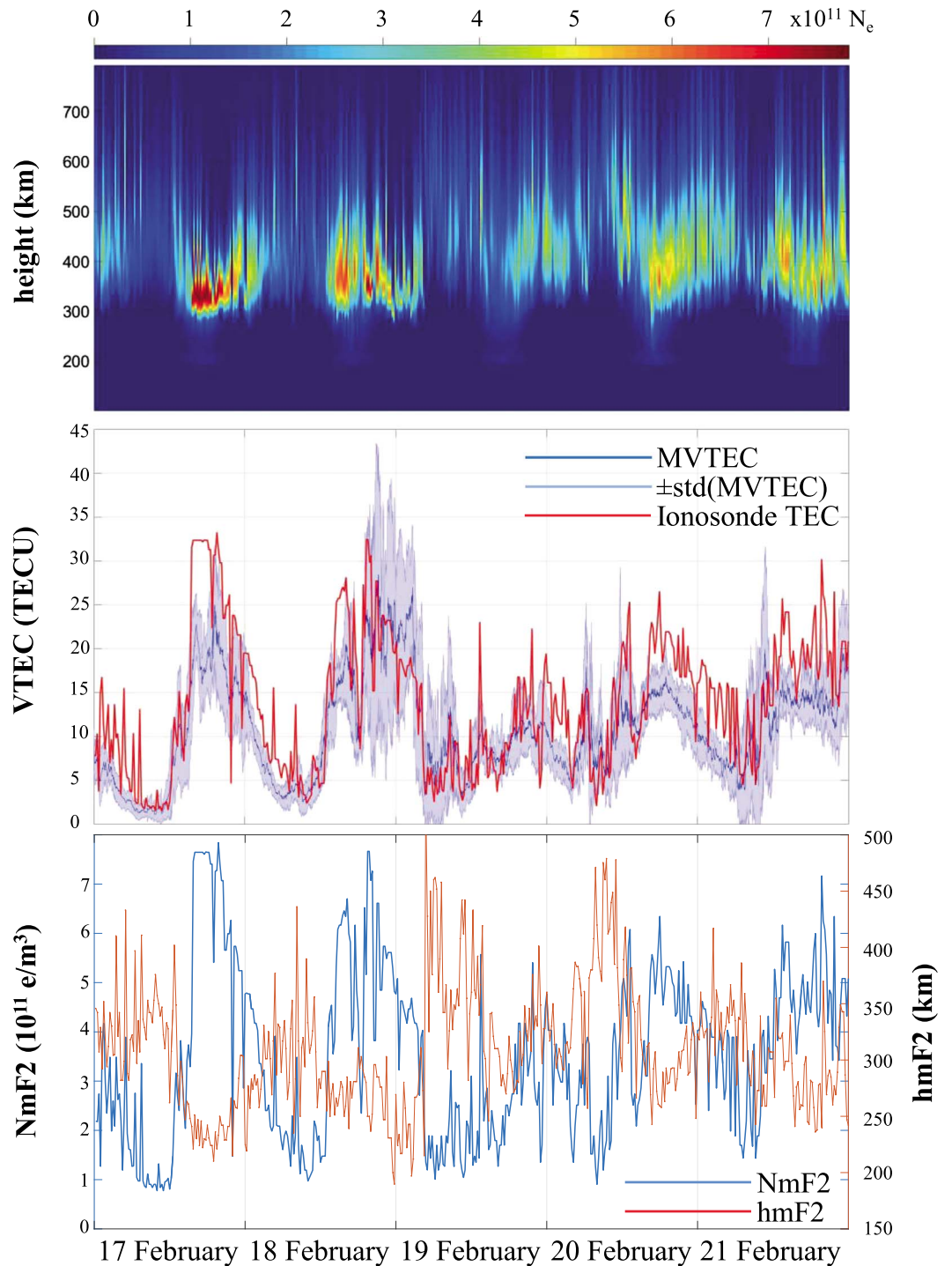
Figure 4. (top) Ionogram-derived profiles showing 5 days of ionospheric vertical N_e distributions observed by a digital ionosonde located at Thule. The measurements were collected at every 15 min. The N_e distributions show that the principal ionized region is the F layer with h_m F_2 typically around 300 km. (middle) MVTEC time series above Thule during the same days as shown in the top image (dark blue line) with the standard deviation of the MVTEC (light blue shading) and the ionosonde-derived TEC (red line). The diurnal ionization cycle in the F layer was disrupted after the first CME arrival. The TEC recovery occurs for several days similarly to the Dst (ring current) recovery (Figure 2). (bottom) N_m F_2 and h_m F_2 time series demonstrating negative correlation.
