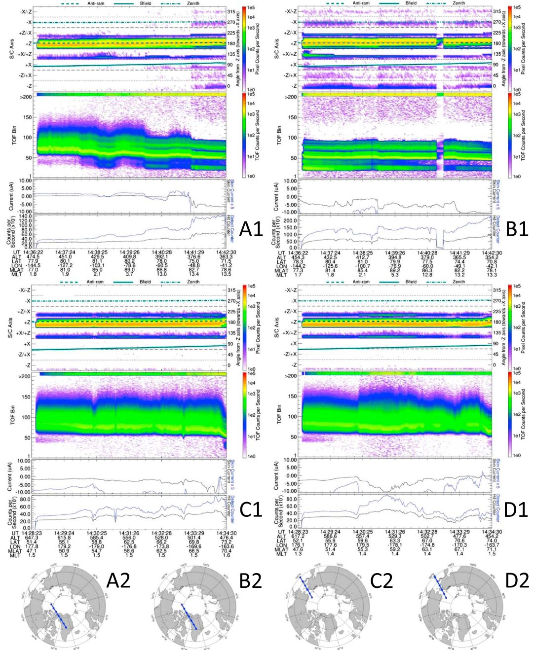
Figure 9. Measurements acquired from four different CASSIOPE passes. A2, B2, C2, and D2 are the ground-tracks referring to the measurements of A1, B1, C1, and D1, respectively. A1 was observed on 17 February, B1 was on 18 February, C1 was on 19 February, and D1 was on 20 February 2014 during near-perigee passes. The spacecraft (S/C) Axis panels show the EA-t spectrograms of averaged ion count rate in the order of pixel sectors and pixel radii within the pixel sector. Antiram, magnetic field, and zenith directions are depicted by dashed, continuous, and dotted lines, respectively. The TOF Bin panel shows the TOF-t spectrogram of the ion count rate. Both at bias voltage of V_{SA} \approx -176 V. The Current panel shows the measured skin current in \mu A and the Counts per Second panel shows the total ion count measured by the detector per second [Yau et al., 2015]. The ground tracks of passes A and B are in Greenland, while C and D are also in the Arctic region at approximately the same latitudes but on the opposite side of the magnetic pole. Unfortunately, other well-collocated passes were not available during this storm event. During all four passes the antiram pixel sector indicated the highest ion count rate, meaning ions were arriving predominantly from the ram direction. Since each of the passes occurred during early afternoon UTC the satellite was flying against the antisunward convection at a relatively low angle each time. The TOF Bin panels on the 19 and 20 show higher values than on the 17 and 18 which indicate the occurrence of heavier (molecular) ion species.
