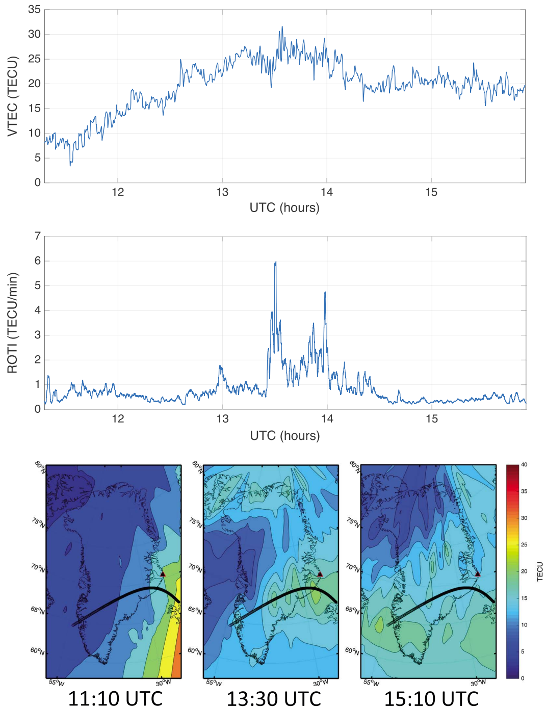
Figure 10. (top) PRN 05 (SVN 50) GPS satellite single-arc (the acronyms stand for pseudorandom noise and space vehicle number respectively), bias-free VTEC values on 19 February 2014. Derived from Scoresbysund station data (its location is marked with black triangle on Figure 10 (bottom)). (middle) ROTI calculated for the same satellite arc. (bottom) Three 2-D TEC maps for the same day as Figures 10 (top) and 10 (middle). We used data from all 18 stations (see Figure 1) at different UTC times. The thick black line is the IPP arc for this satellite for the time span presented in Figures 10 (top) and 10 (middle).
