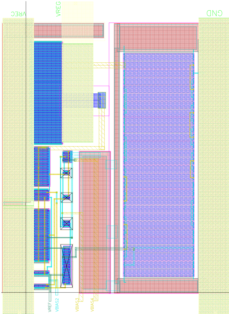
Figure B.2: Layout of LDO
