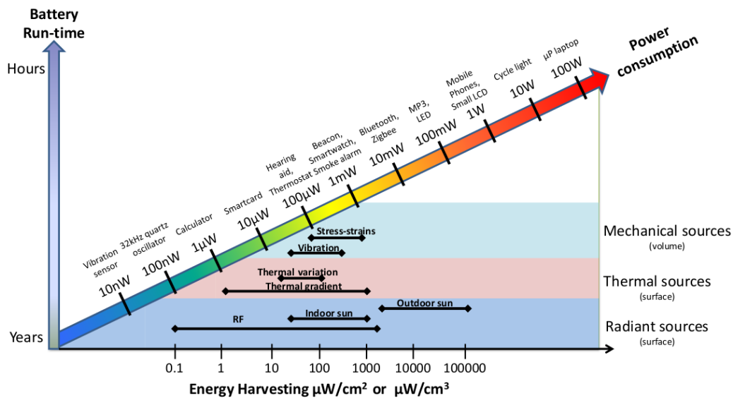
Figure 2.2: Power density of energy sources and consumption of electronic devices [5]
