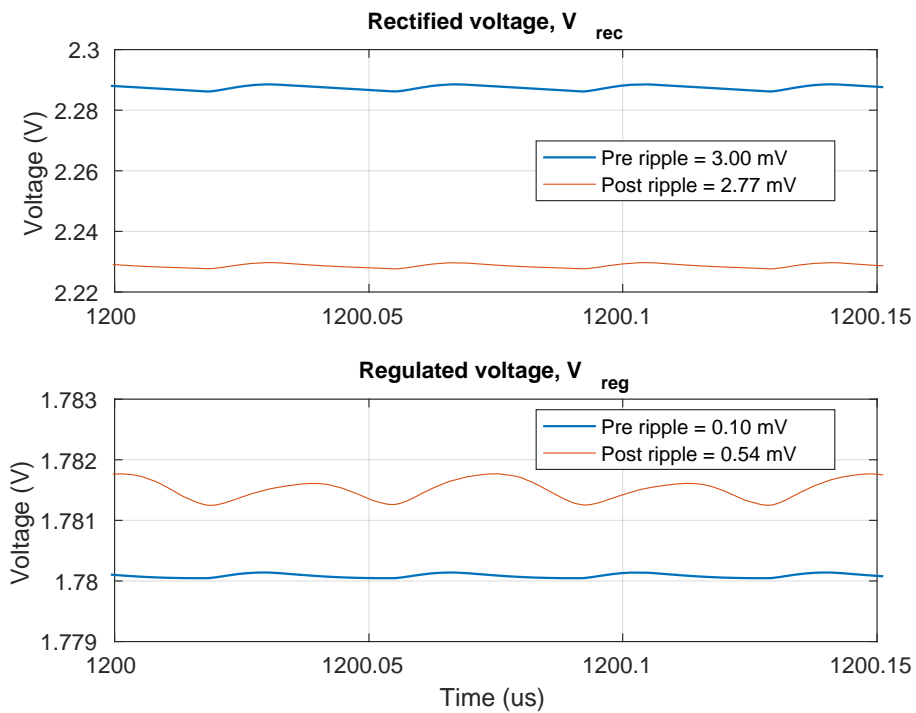
Figure 6.11: Ripple in V_{rec} and V_{reg}
