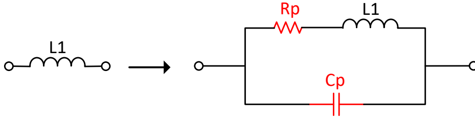
Figure 5.2: Real antenna model
