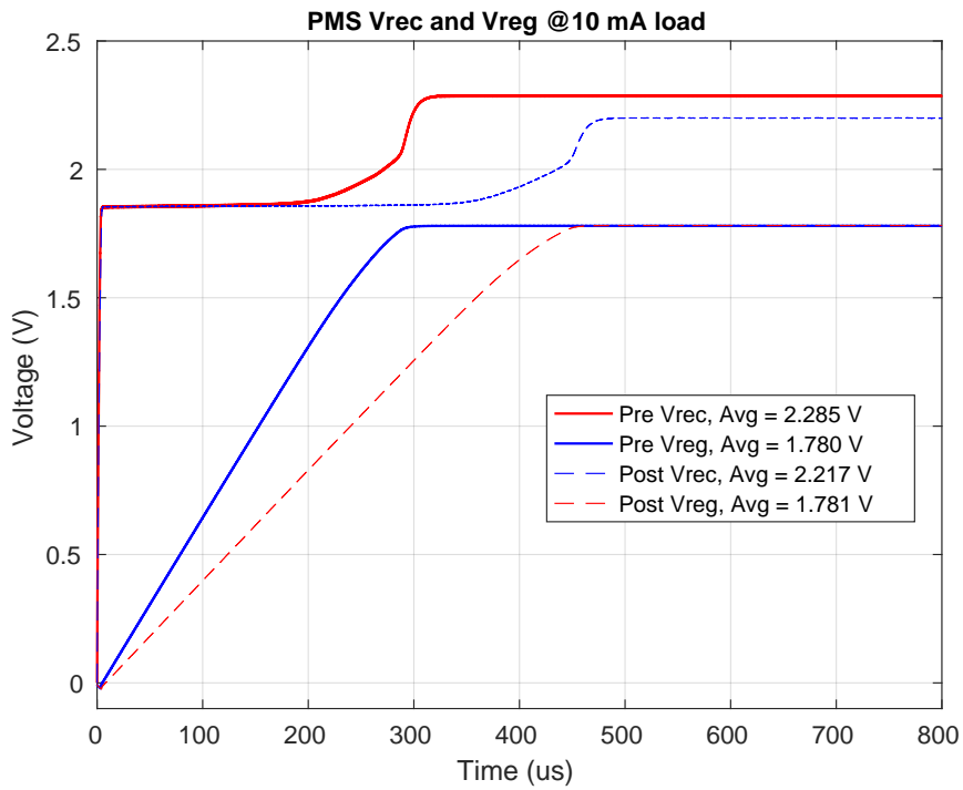
Figure 6.5: V_{rec} and V_{reg} voltages of PMS
