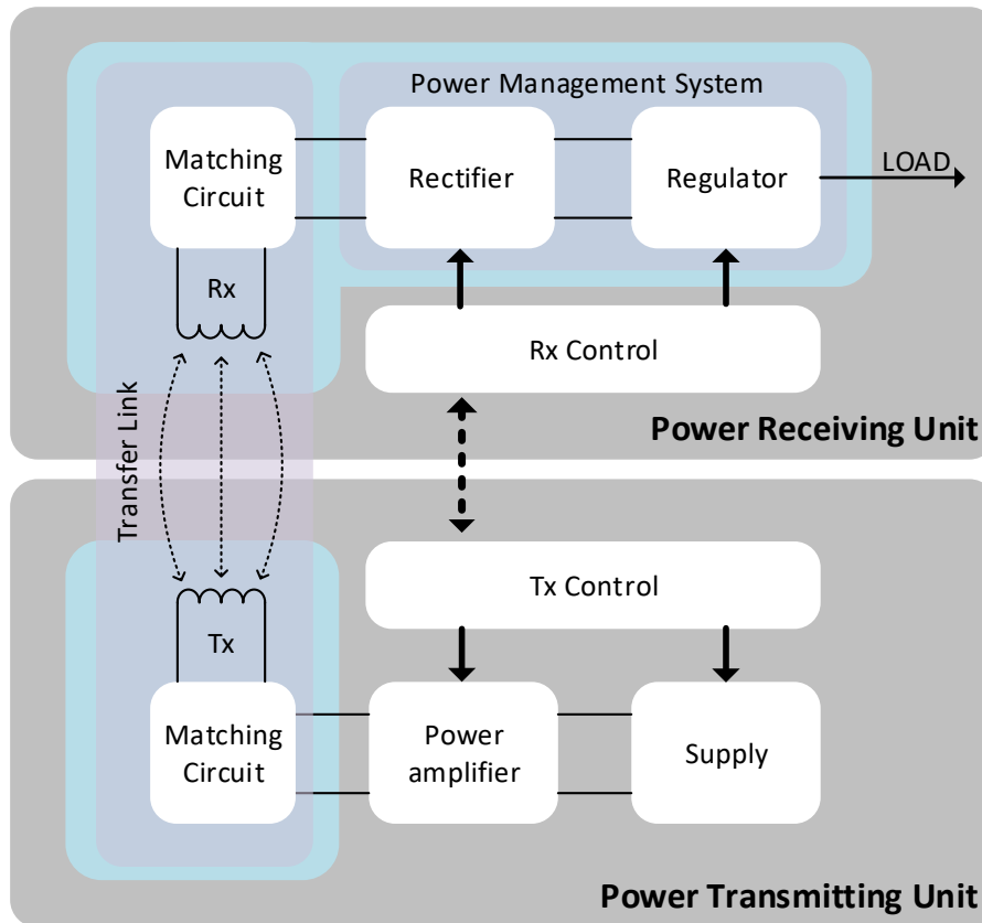
Figure 6.1: WPT block diagram
