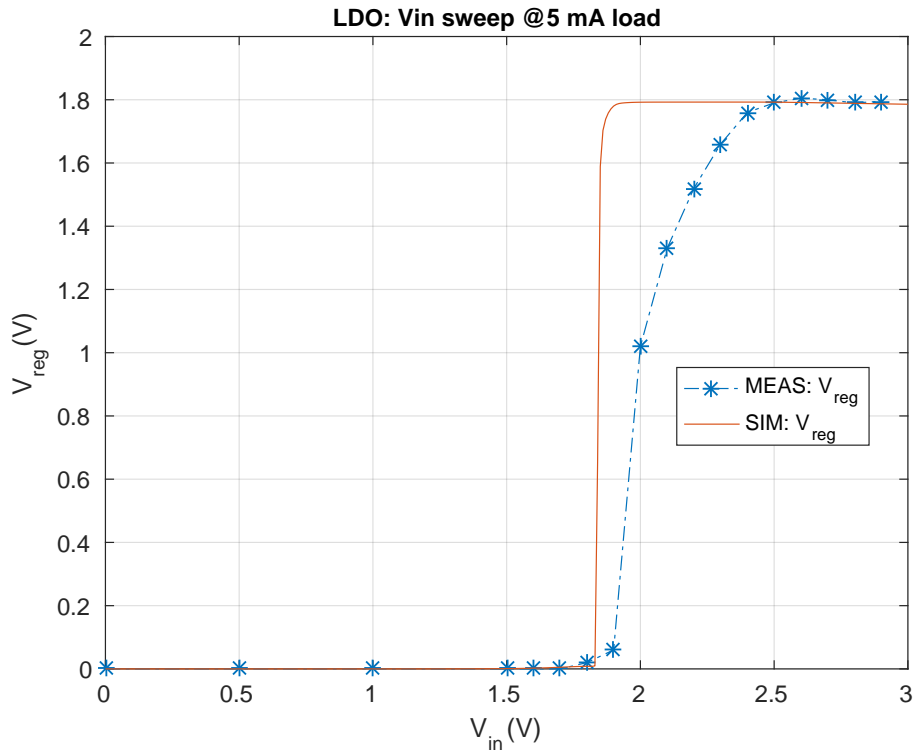
Figure 7.6: LDO input sweep for 5 mA load
