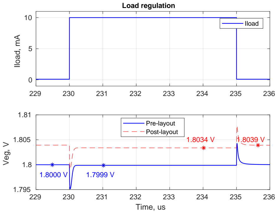
Figure 4.5: LDO step load regulation
