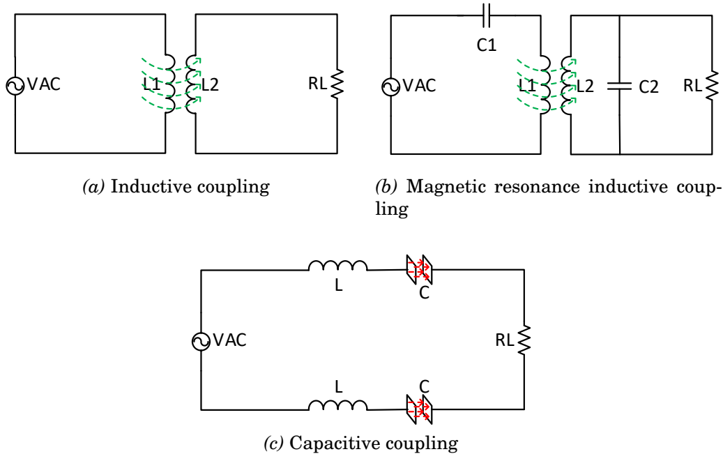
Figure 2.3: Near-field coupling models
