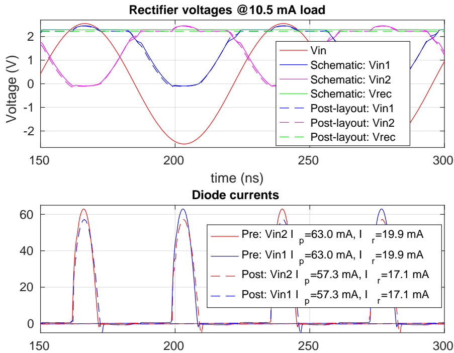
Figure 3.7: Voltage and current waveforms of the rectifier
