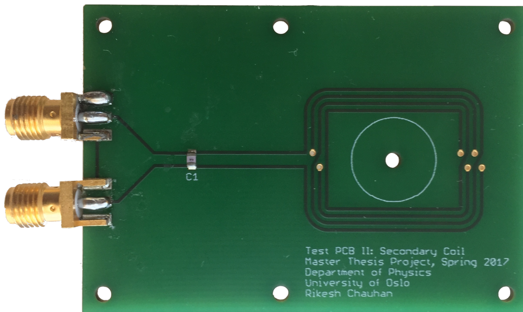
Figure D.4: Secondary antenna PCB
