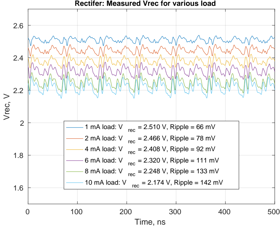
Figure 7.5: Measured rectifier output for various load
