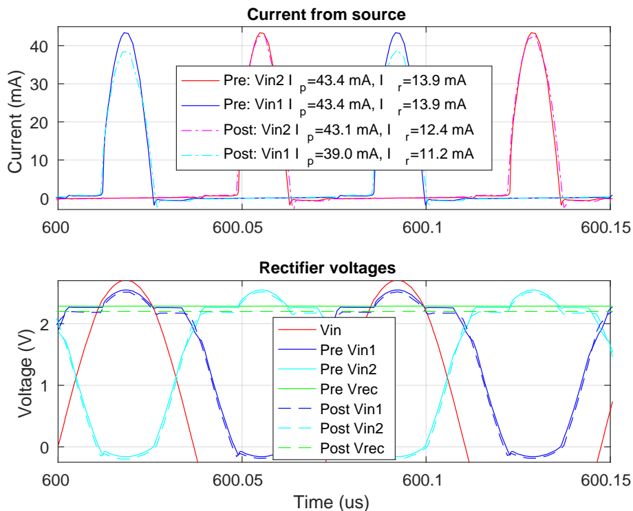
Figure 6.7: Current and power consumption
