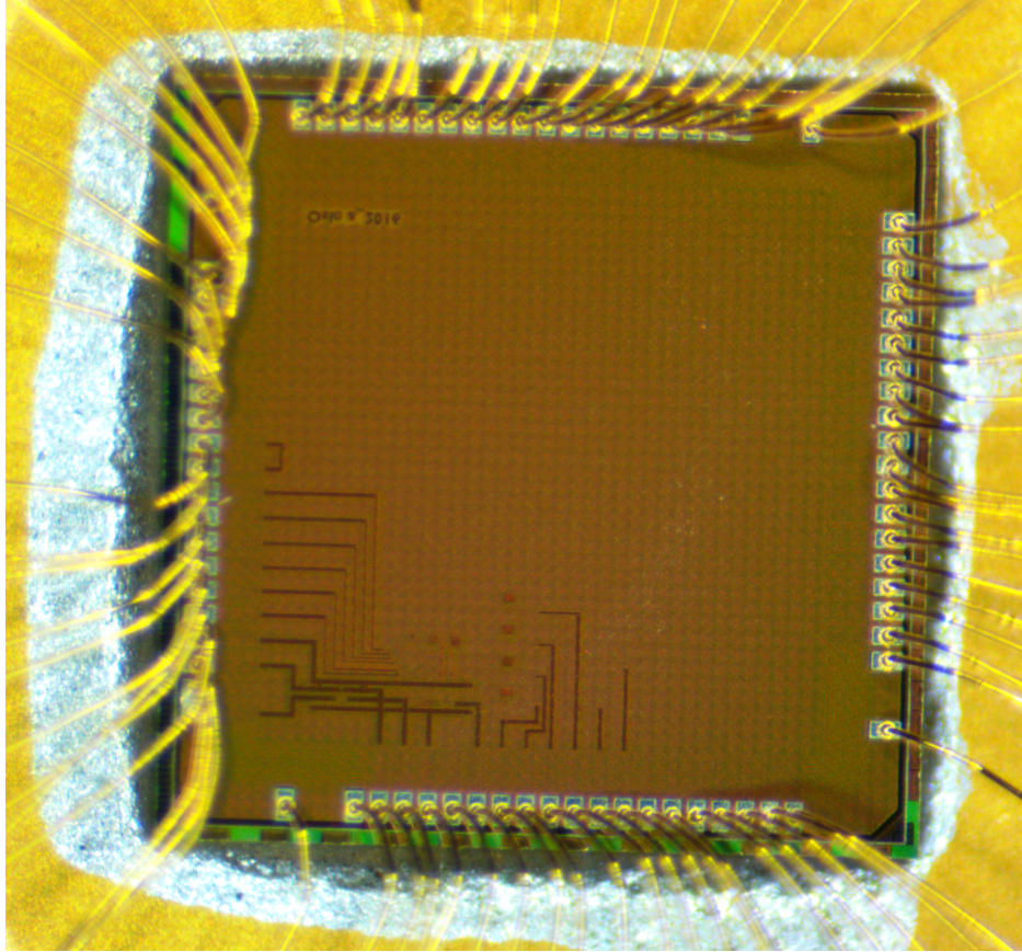
Figure 7.1: Micrograph of PMS chip
