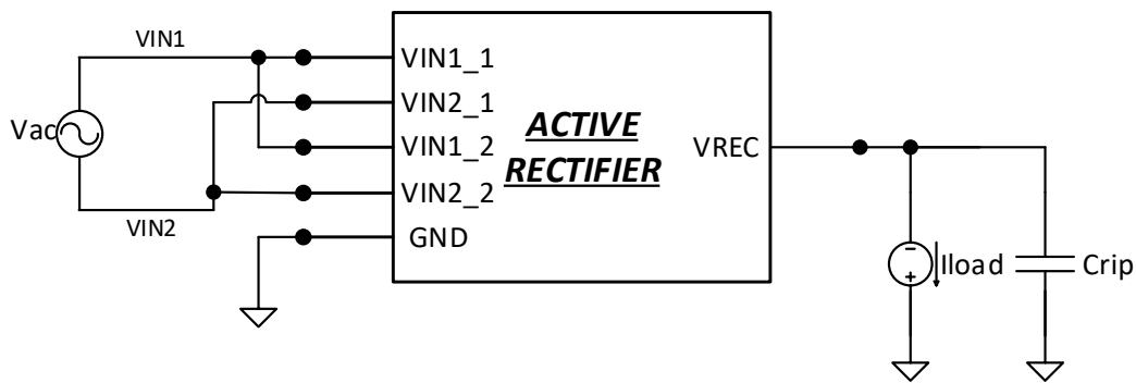
Figure 3.4: Testbench for rectifier
