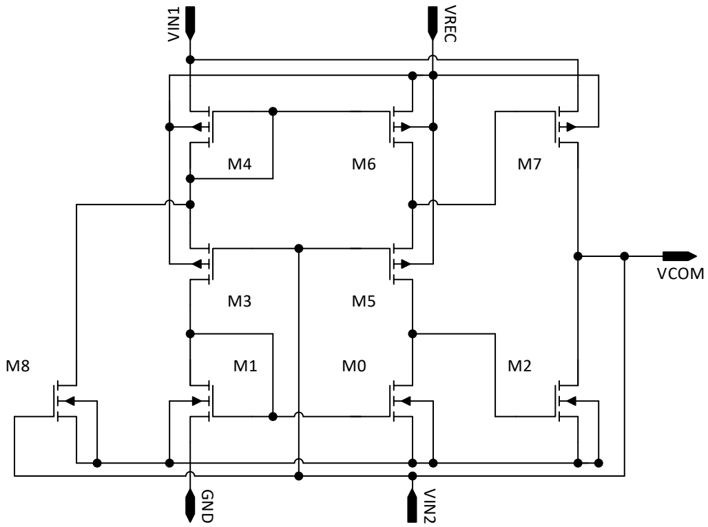
Figure 3.3: Comparator circuit, RCC
