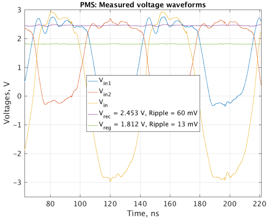
Figure 7.8: PMS performance
