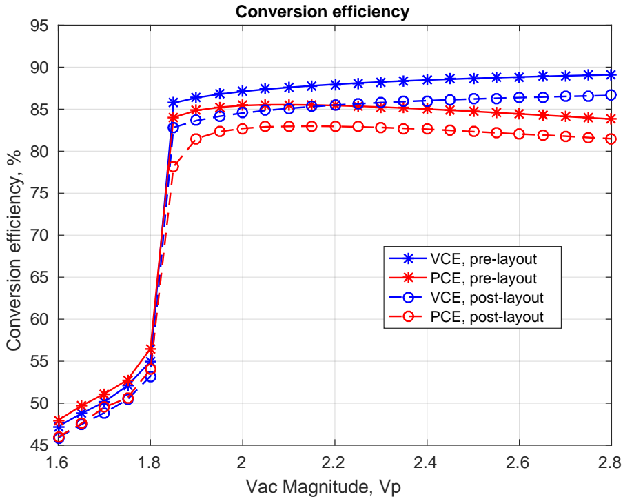
Figure 3.8: Voltage and power conversion efficiency
