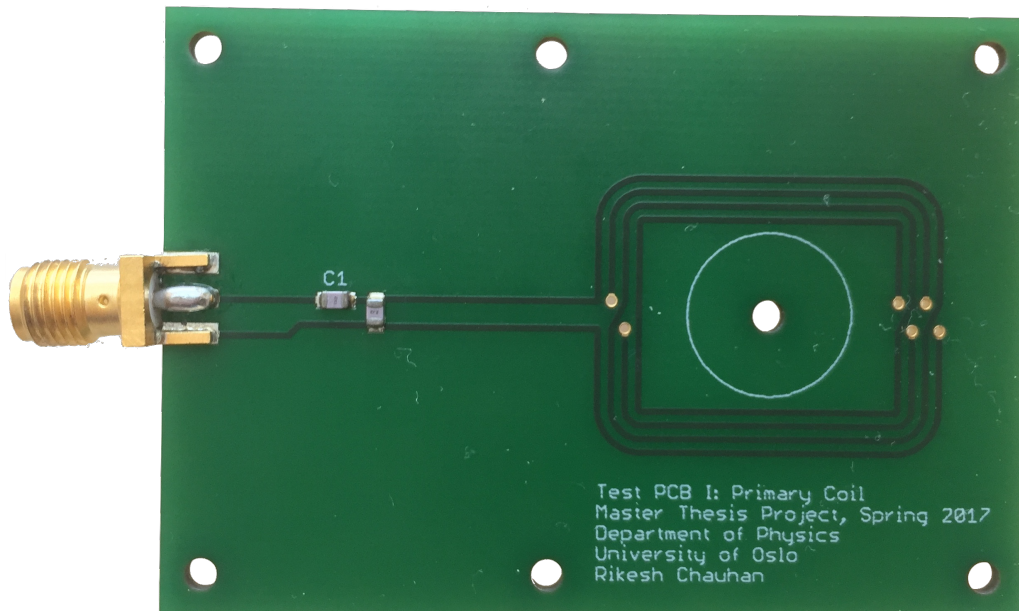
Figure D.2: Primary antenna PCB
