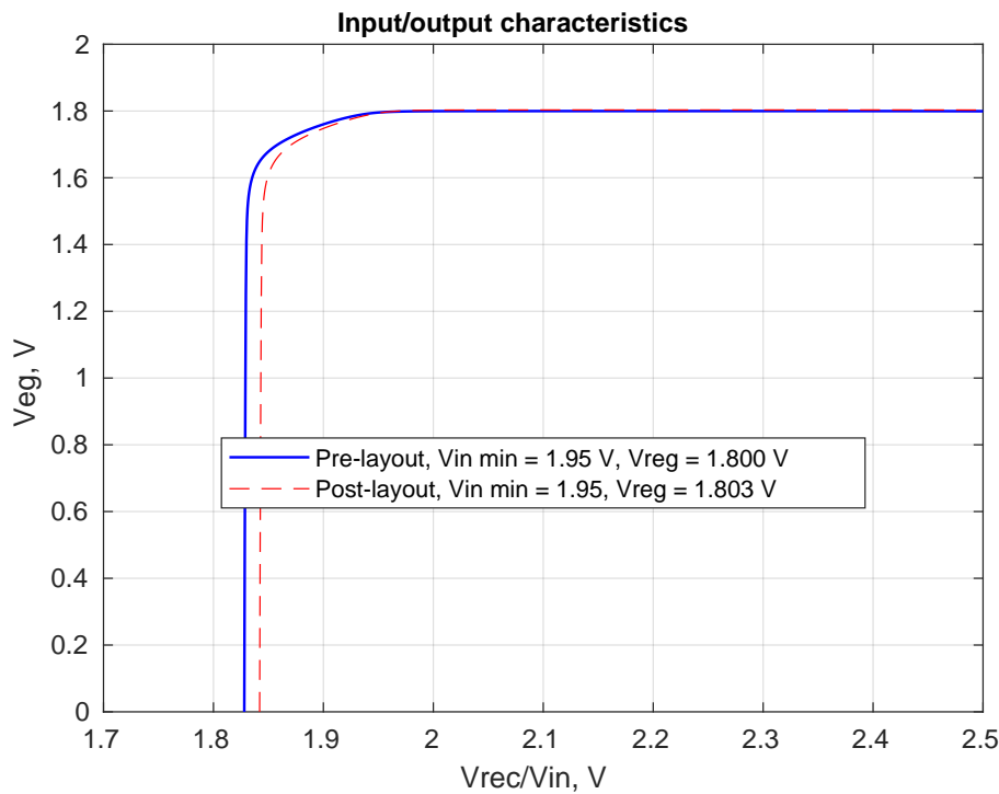
Figure 4.7: Regulated voltage with supply variation
