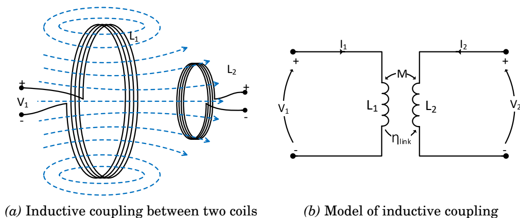
Figure 5.1: Inductive coupling
