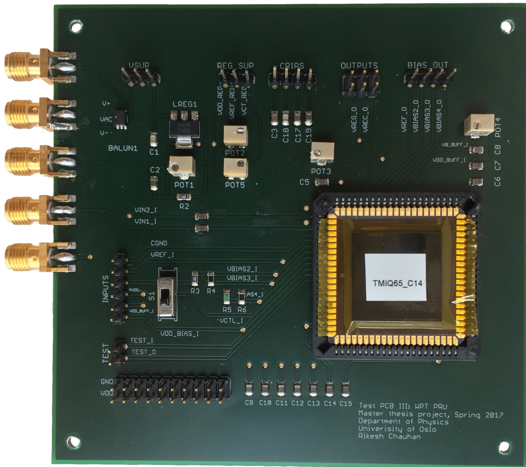
Figure D.7: Test PCB board
