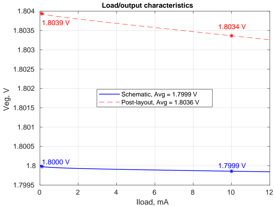
Figure 4.8: Regulated voltage with load variation
