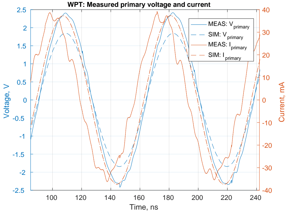
Figure 7.10: WPT 5 mm coupling: Voltage and current at primary coil
