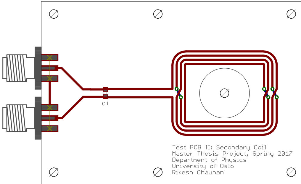
Figure D.3: Secondary antenna
