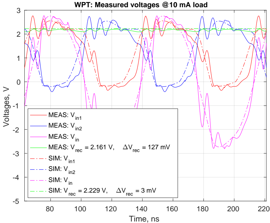
Figure 7.9: WPT from 5 mm coupling: voltage waveform
