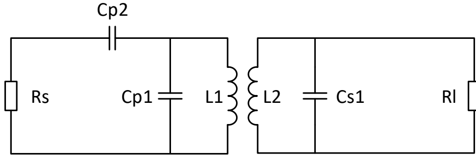
Figure 5.5: Resonant coupled inductive link
