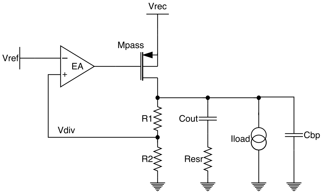
Figure 4.1: Generic LDO with pMOS pass device
