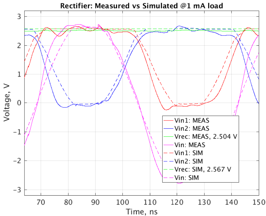
Figure 7.4: Measured rectifier waveform for 1 mA load
