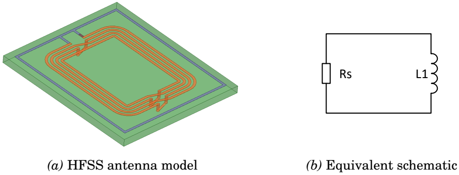
Figure 5.3: Antenna model
