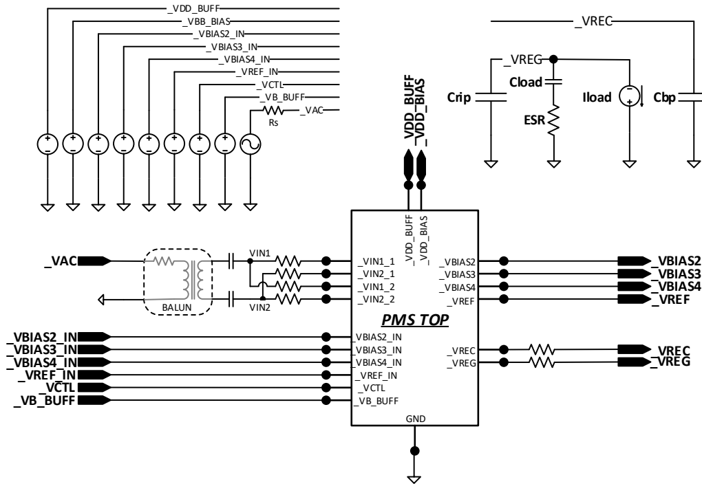
Figure 6.3: Test bench for PMS simulation
