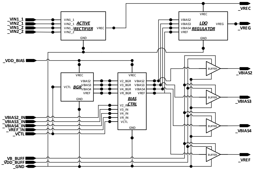
Figure 6.2: WPT PMS implementation
