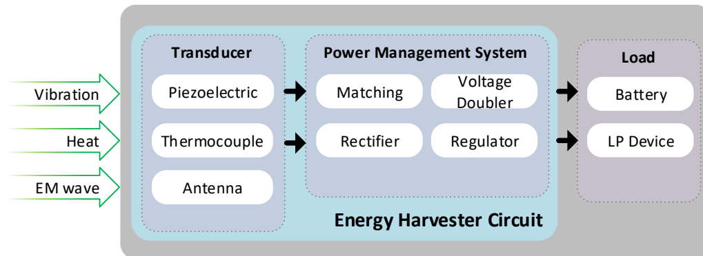
Figure 2.1: Functional block diagram of energy harvesting system
