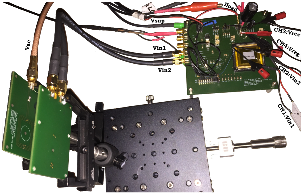
Figure 7.2: Measurement setup
