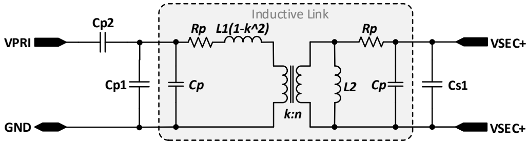
Figure 6.8: Lumped model of inductive link
