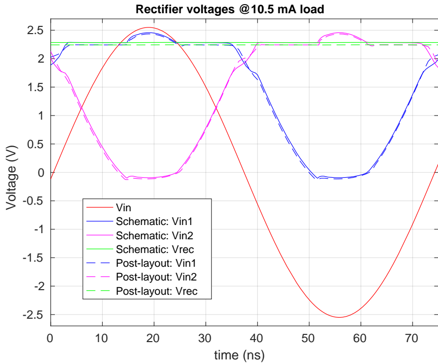
Figure 3.5: Voltages waveform for pre and post layout
