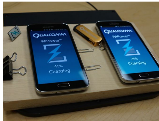
(b) Qualcomm mobile phone charger with foreign object detection feature
