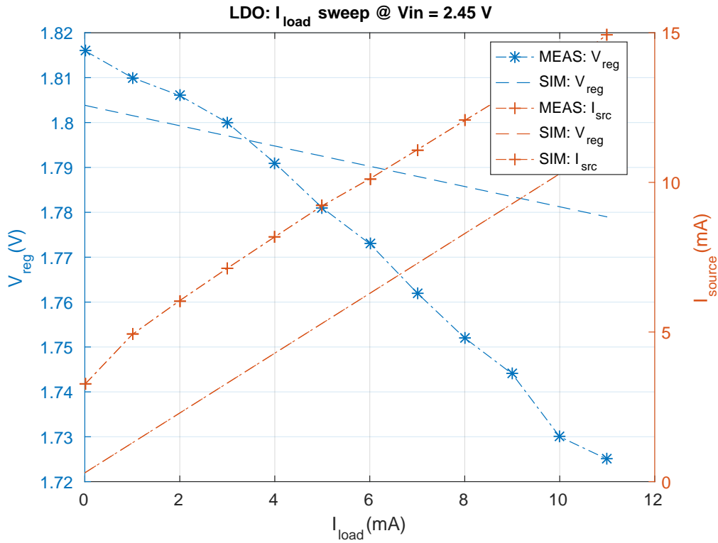
Figure 7.7: LDO load sweep
