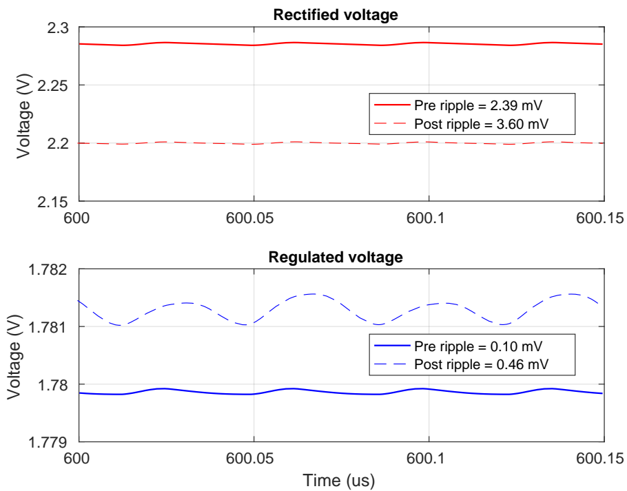
Figure 6.6: Ripple in V_{rec} and V_{reg}
