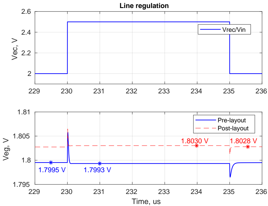
Figure 4.6: LDO step line regulation
