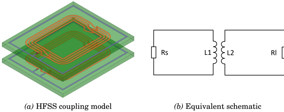
Figure 5.4: Antenna coupling model
