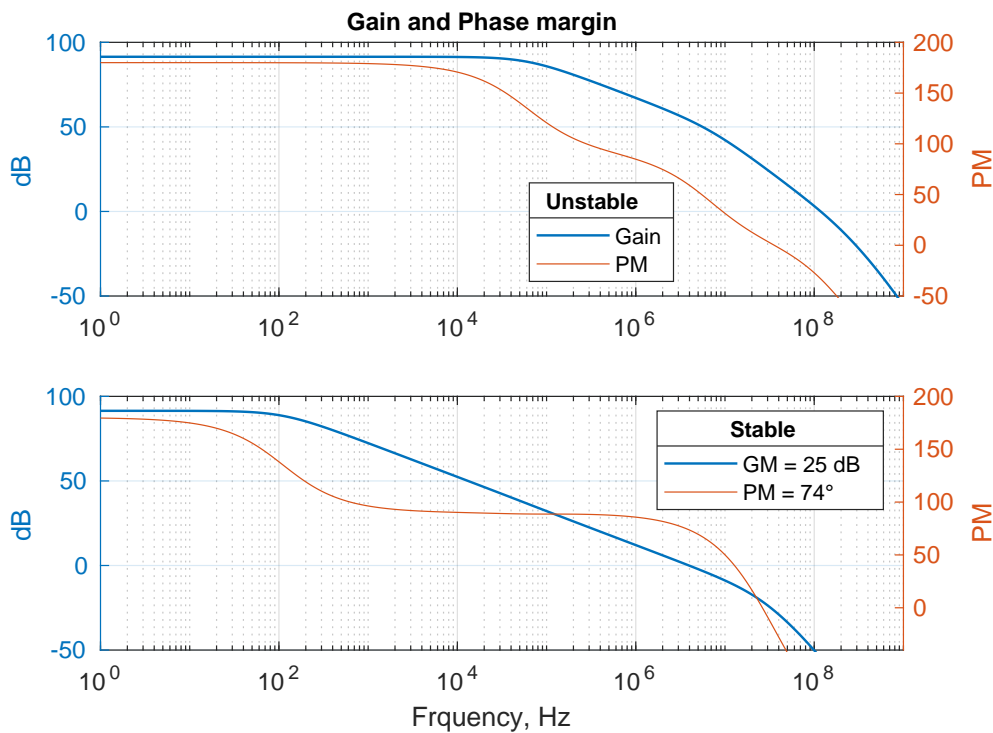
Figure 4.9: LDO stability before and after compensation
