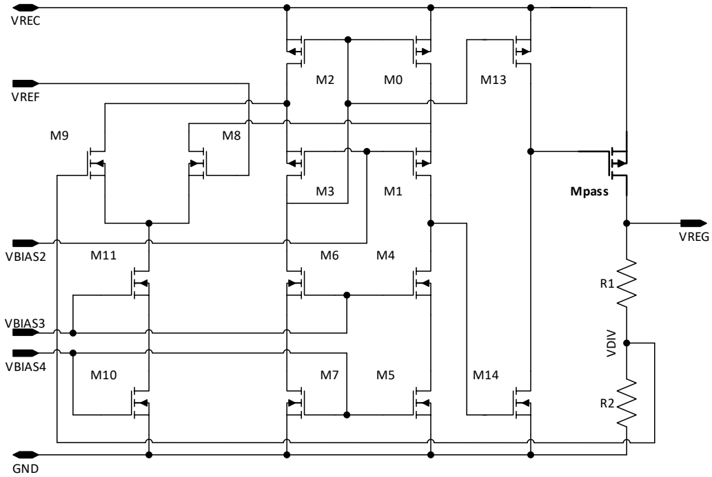
Figure 4.2: CMOS implementation of LDO
