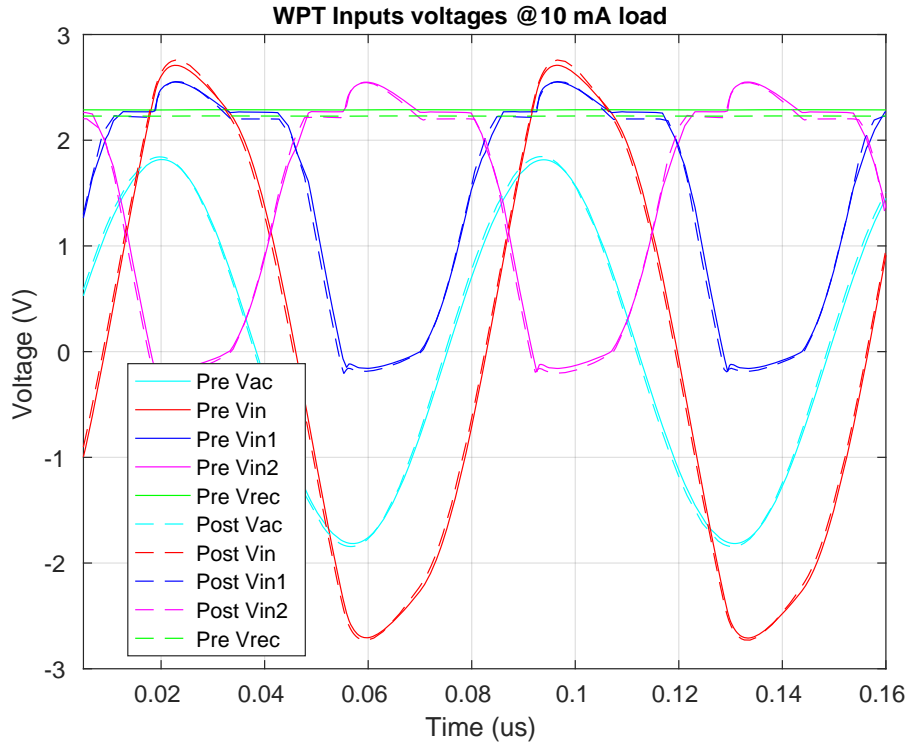
Figure 6.9: Input voltage waveforms
