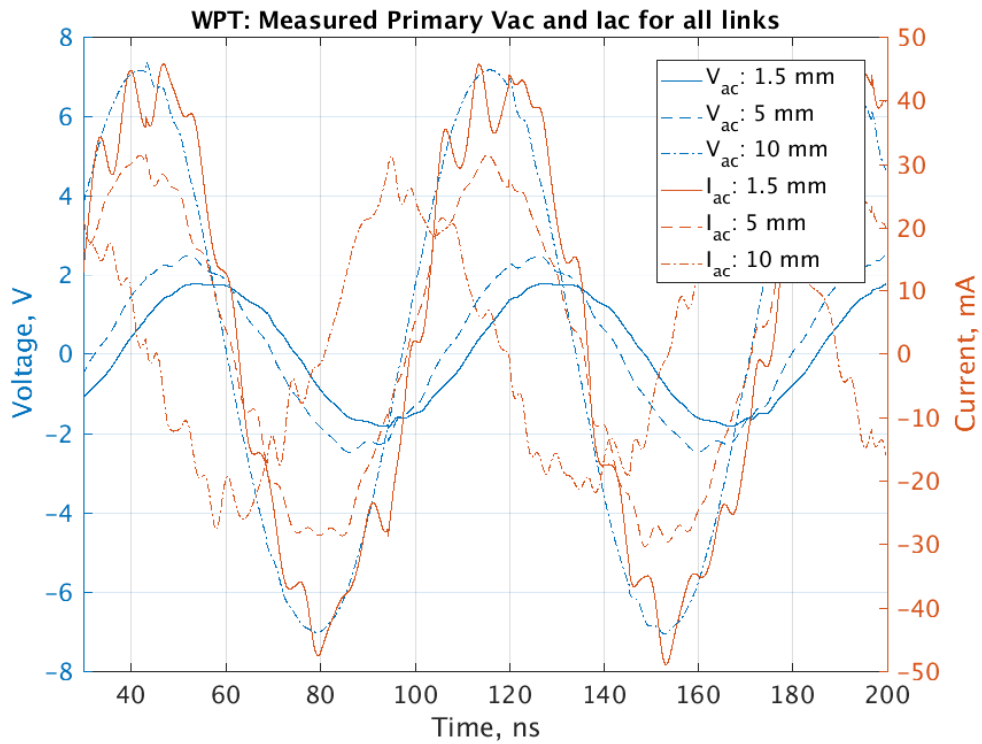
Figure 7.11: Primary voltage and current for various inductive link
