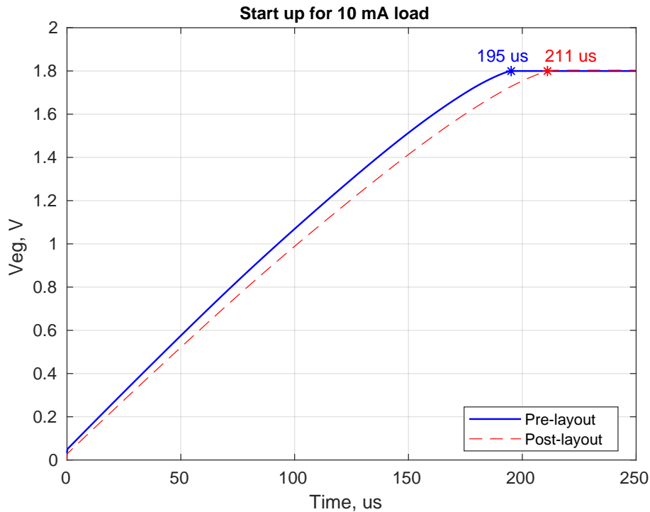
Figure 4.4: LDO transient simulation
