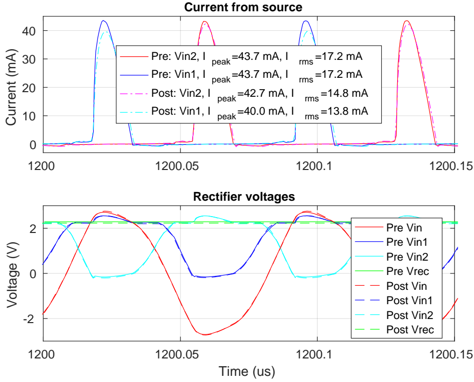
Figure 6.13: Diode current and voltages
