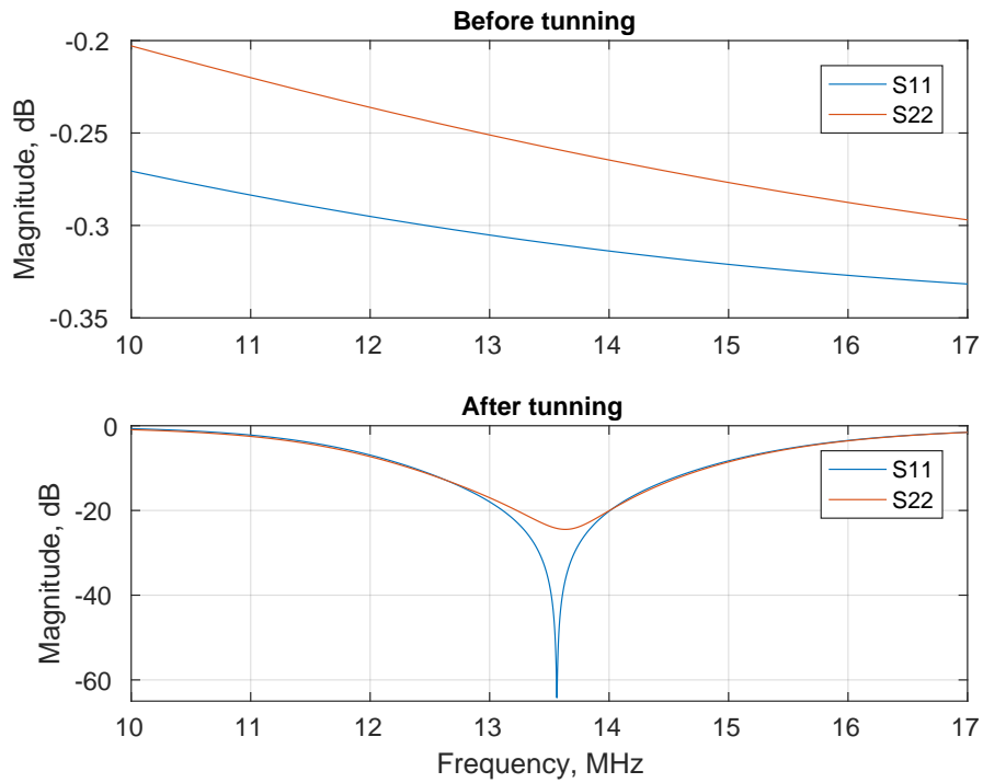
Figure 5.6: Link reflection loss before and after tuning
