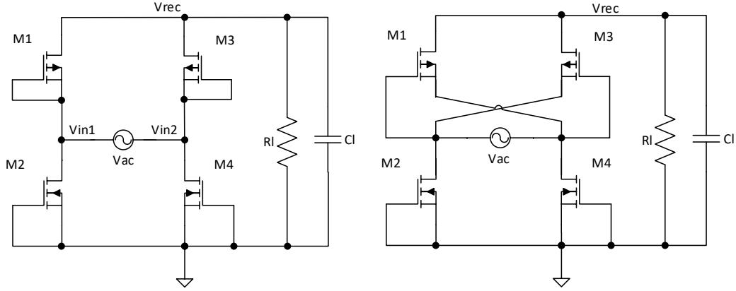
(a) Conventional full wave bridge rectifier (b) Gate cross coupled full wave rectifier
