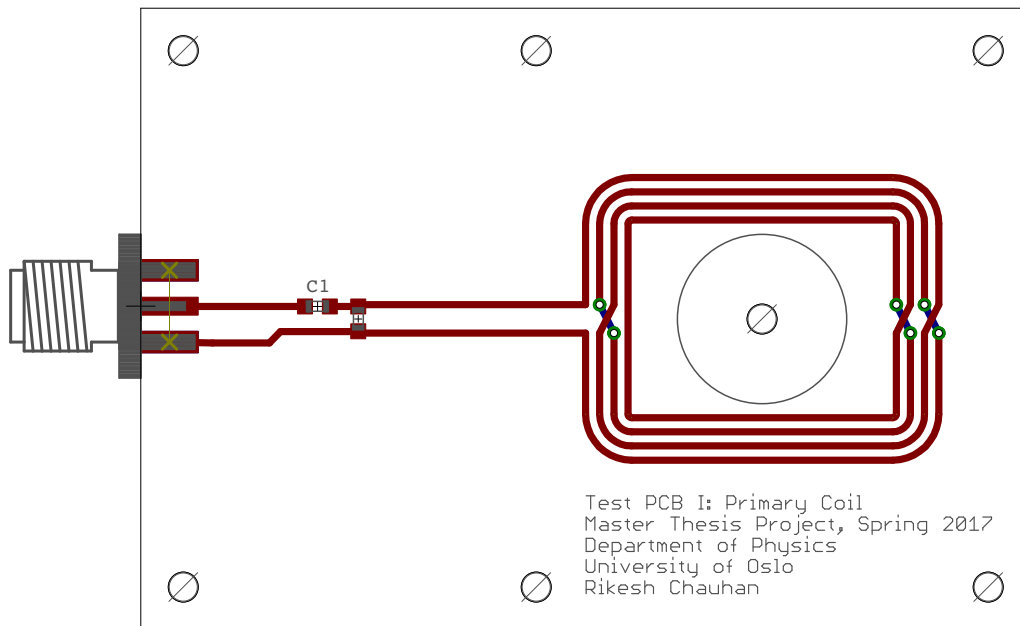
Figure D.1: Primary antenna layout
