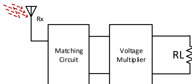
Figure 2.4: Far-field harvesting model
