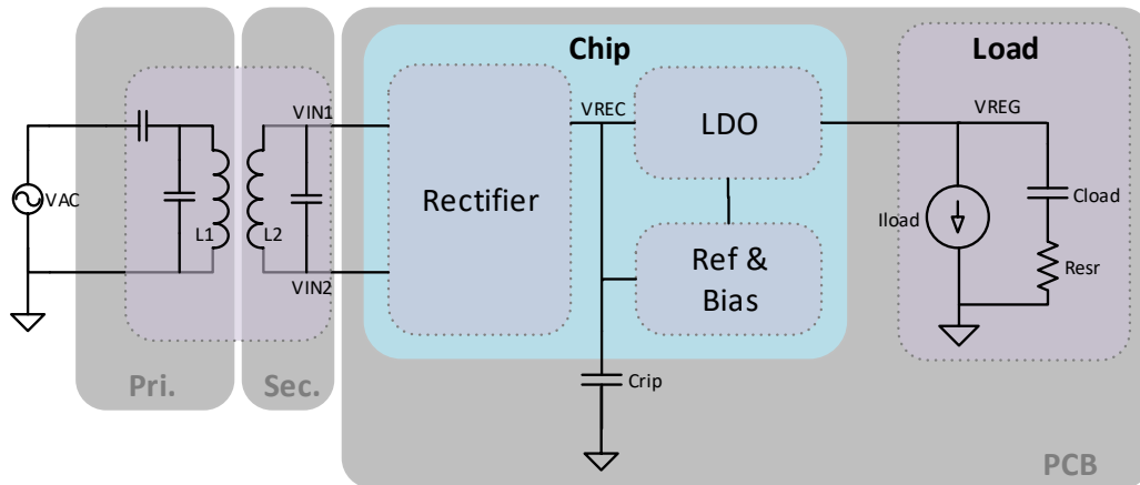
Figure 2.8: Functional block diagram of complete design
