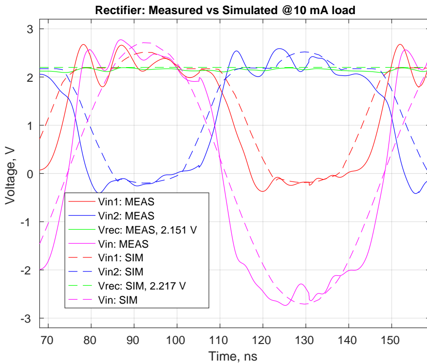
Figure 7.3: Measured rectifier waveform for 10 mA load
