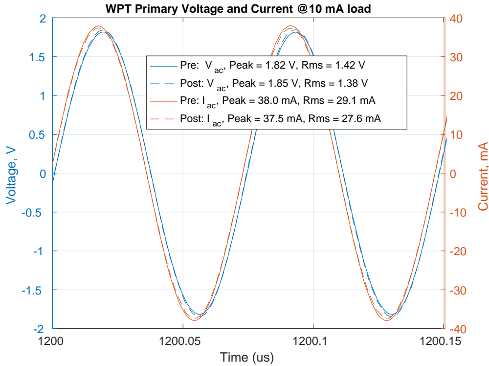
Figure 6.12: Primary voltage and current
