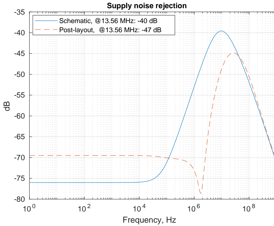
Figure 4.10: PSSR performance
