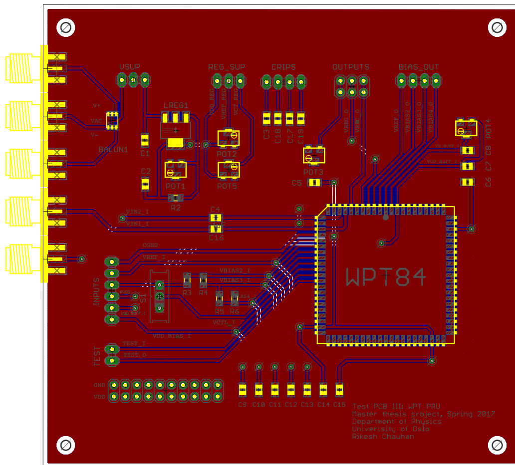
Figure D.6: Test PCB board layout
