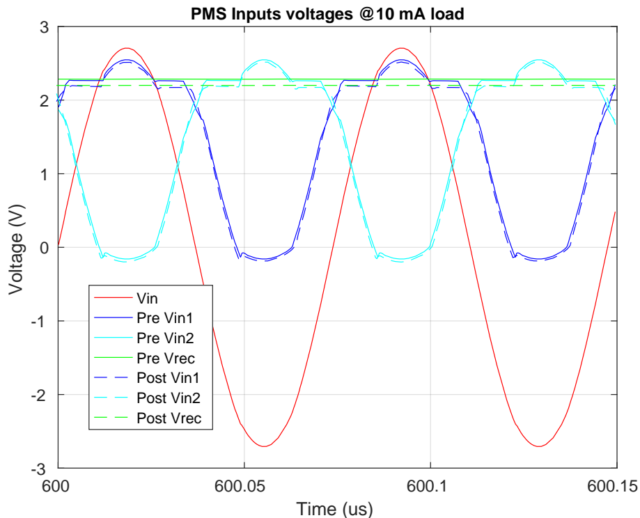
Figure 6.4: Input voltage waveform of PMS
