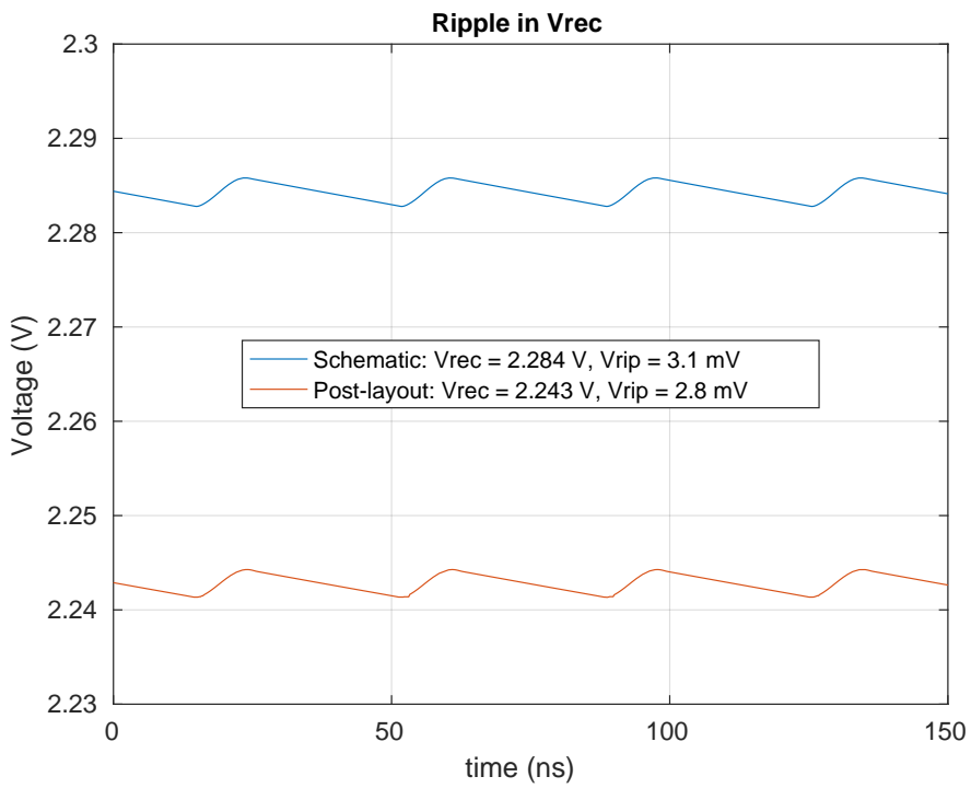
Figure 3.6: Rectified output for pre and post layout
