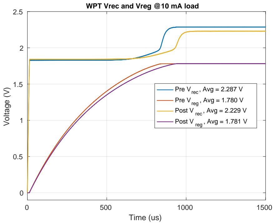
Figure 6.10: V_{rec} and V_{reg} voltages
