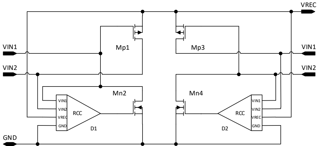
Figure 3.2: Gate cross coupled full wave active rectifier
