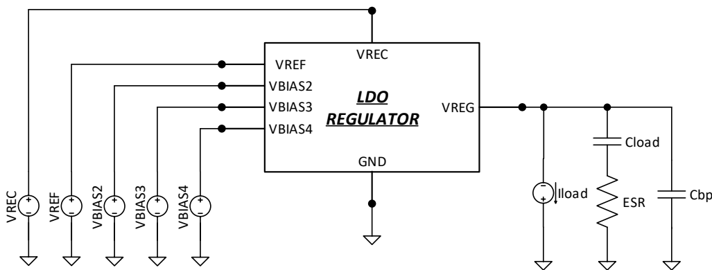
Figure 4.3: LDO testbench setup
