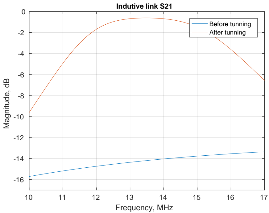
Figure 5.7: Link gain before and after tuning
