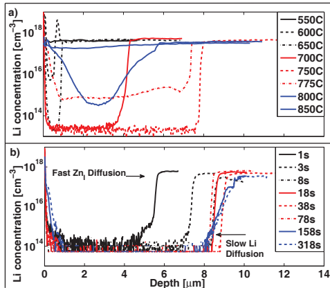
FIG. 3: Li concentration versus depth profiles as measured upon (a) isochronal (30 min) and (b) isothermal ( 800^\circ\text{C} ) anneals of H_{Zn} samples.
