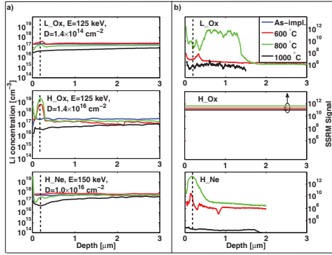
FIG. 2: (a) Li concentration versus depth profiles as measured by SIMS and (b) corresponding SSRM signals for O and Ne ion implanted samples. The annealing time was 1 hour for all the temperatures. The dashed lines indicate R_p of the implanted ions ( \sim 180 nm). The data for the H_Ox samples are above the range accessible by our setup.
