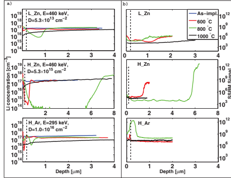
FIG. 1: (a) Li concentration versus depth profiles measured by SIMS and (b) corresponding SSRM signals for Zn and Ar ion implanted samples. The annealing time was 1 hour for all the temperatures. The dashed lines indicate R_p of the implanted ions ( \sim 180 nm). Notice the difference in depth scale for sample H_Zn due to the deep Li redistribution.
