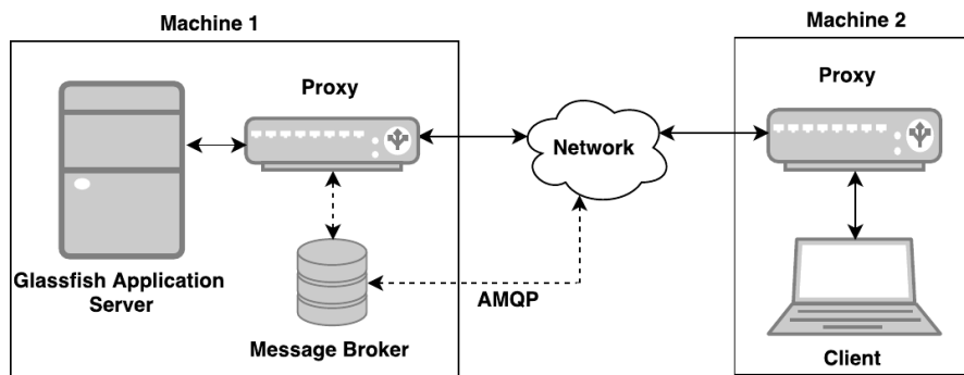
Figure 6.6: Test setup
