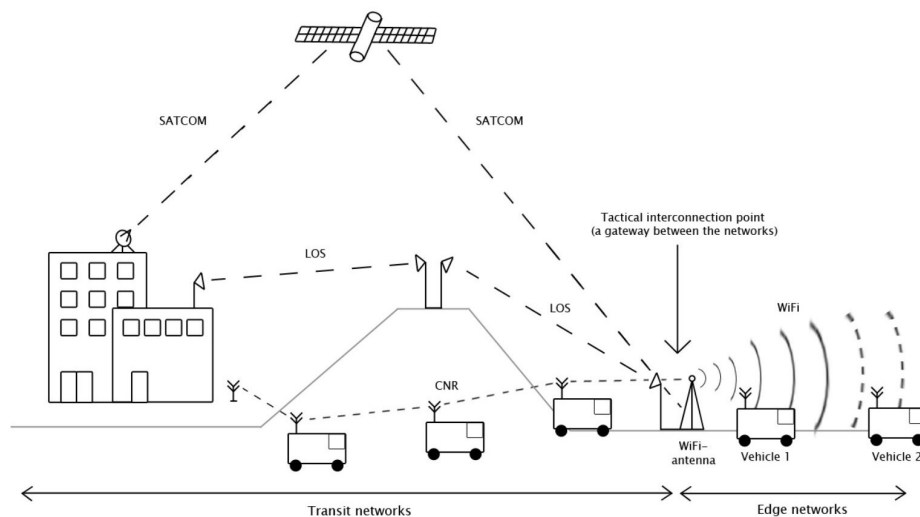
Figure 6.1: Overview of tested networks (from [50])
