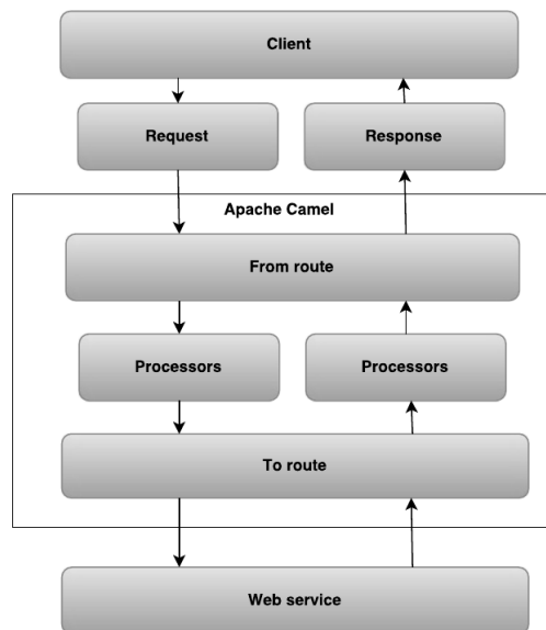
Figure 5.4: Example of a Camel route
