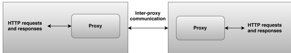
Figure 5.2: Solution concept
