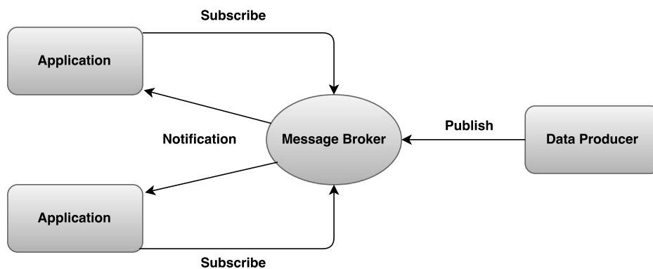
Figure 2.1: Message Brokers
