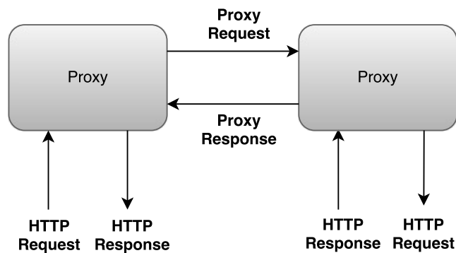
Figure 5.5: Proxy routes
