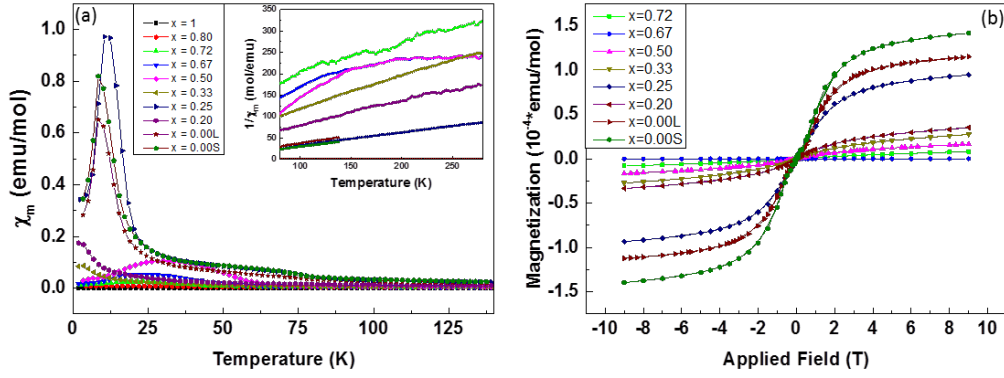
Figure 6. Left; temperature dependence of the magnetic susceptibility \chi_m(T) for \text{La}_4(\text{Co}_{1-x}\text{Ni}_x)_3\text{O}_{10} 0.00 \leq x \leq 1.00 ; x compositions are x = 0.00\text{S}, 0.00\text{L}, 0.20, 0.25, 0.33, 0.50, 0.67, 0.72, 0.80, and 1.00 ; insert shows \chi^{-1}(T) . Right; M(H) data for fields up to 9 T at a temperature of 4 K for all concentrations except x = 0.80 to 1.00 .
