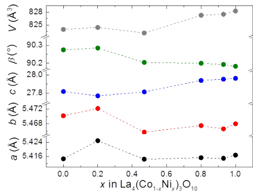
Figure 1. Unit cell dimensions for \text{La}_4(\text{Co}_{1-x}\text{Ni}_x)_3\text{O}_{10} at ambient temperature, space group P2_1/a .
