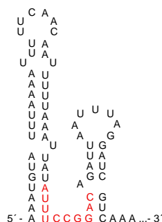
Figure 1-6: The 5'UTR of a Chlamydomonas rbcL transcript. Nucleotides in positions +1 to +69 relative to start of transcription. The cis-acting stability element (nucleotides +38 to +47) shown in red.
