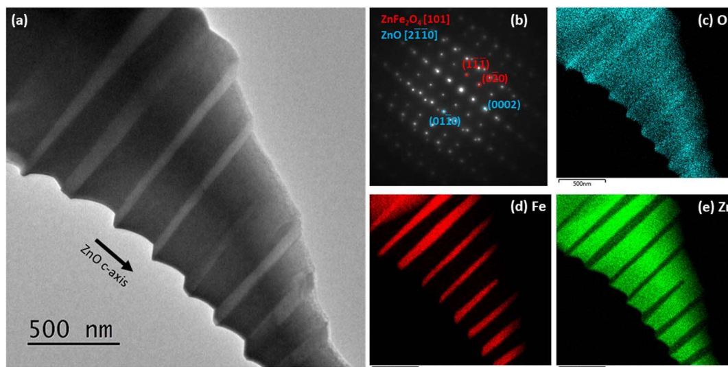
Fig. 2 (a) Bright field STEM image from the nanocomposite sample, taken along the ZnO- [2\bar{1}\bar{1}0] -projection. (b) Indexed SAED pattern from a large part of the area in (a), showing diffraction from both the ZnO matrix and the \text{ZnFe}_2\text{O}_4 NPs. (c)–(e) STEM EDS maps showing an accumulation of Fe and a depletion of Zn at the \text{ZnFe}_2\text{O}_4 NPs, compared to the ZnO matrix.
