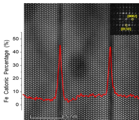
Fig. 4 STEM-HAADF image of the IDB sample along the ZnO- [2\bar{1}\bar{1}0] projection. The inset shows the corresponding FFT. The EDS profile of Fe in cationic percentage is superimposed on the HAADF image. The EDS signal was collected from the entirety of the displayed area, and the Fe-signal was averaged vertically to produce the superposed line profile.
