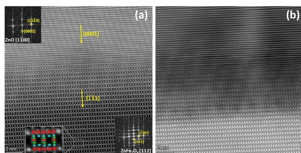
Fig. 3 High resolution (a) STEM-HAADF and (b) STEM-ABF images of the interface between a \text{ZnFe}_2\text{O}_4 NP and the ZnO matrix in the nanocomposite sample. Insets show FFTs from the corresponding areas and a schematic representation of the atomic structure of \text{ZnFe}_2\text{O}_4 overlaid on the magnified HAADF image from the \text{ZnFe}_2\text{O}_4 particle (Zn in green, Fe in red, and O in blue). Yellow arrows indicate the directions of the lattice matching.
