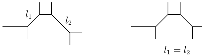
FIGURE 7. Local pictures of tropicalized quartics. An unexpected alignment of two vertices is depicted on the right. For a generic quartic, as shown on the left, the two lengths l_1 and l_2 are different.
