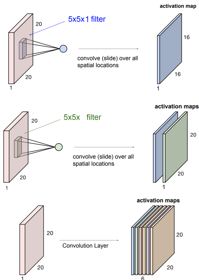
Figure 8.2: Illustration of the convolutional process. The figure has been adapted from Lecture Notes in the course IN5400 from 2021, with attribution to Andreas Kleppe [35].
