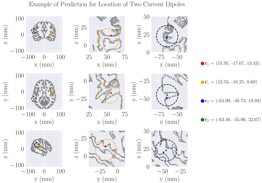
Figure 9.4: Depiction of prediction and true value of the locations of two current dipoles within a sample from the test data set.
