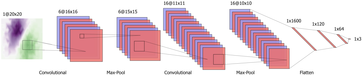
Figure 8.3: Architecture of the Convolutional Neural Network for localizing single current dipoles.
