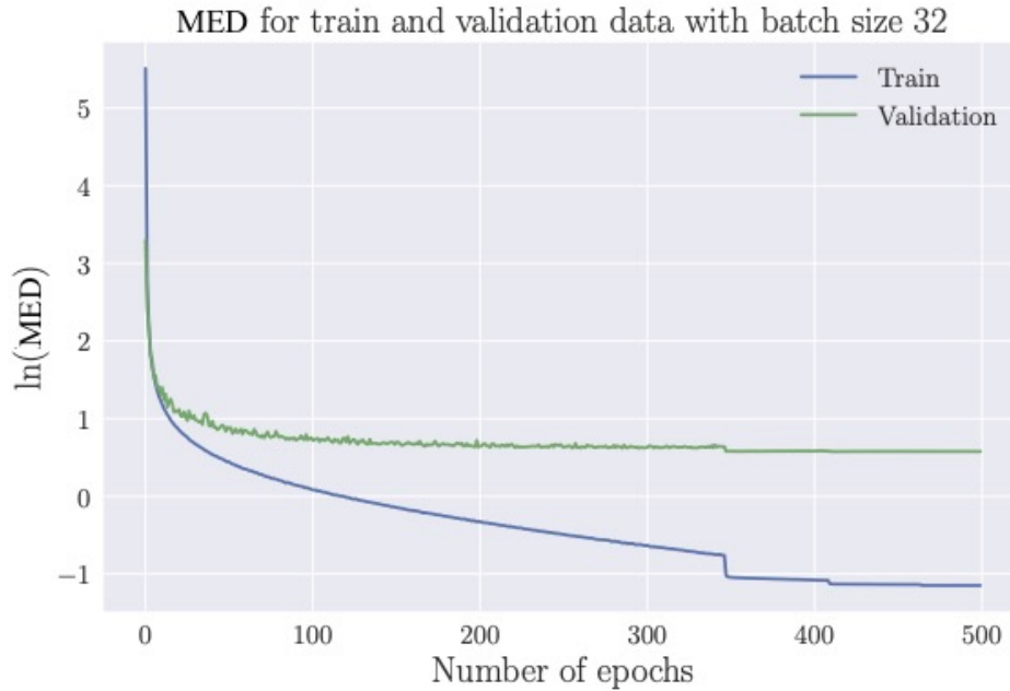
Figure 7.2: Training- and validation MED loss for the fully connected feed-forward (FCNN) neural network with 50,000 samples.
