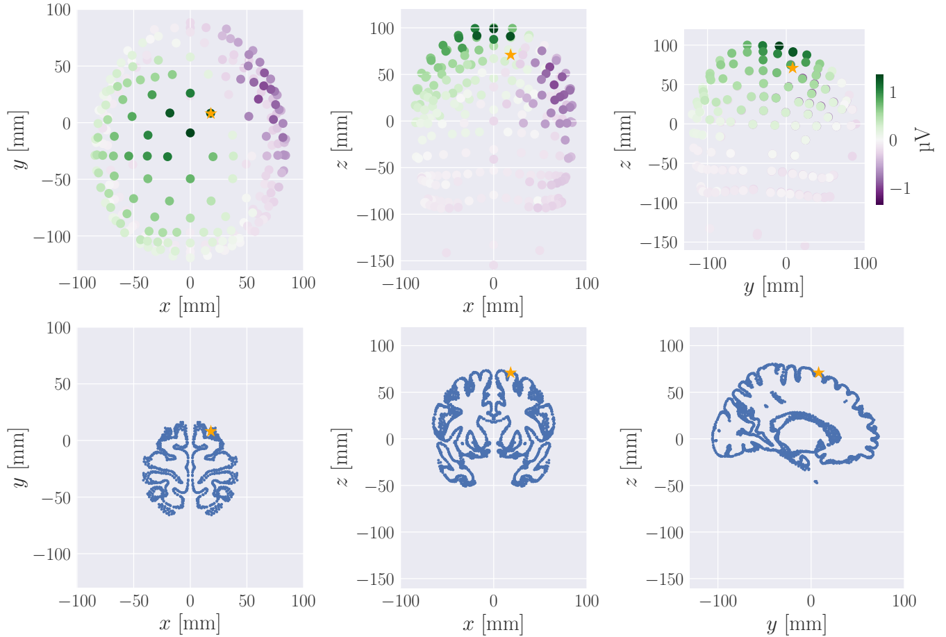
Figure 4.1: EEG measurements for a sample containing one single current dipole source at an arbitrary position within the cerebral cortex. Noise is added to the EEG signal. The EEG measure is seen from both sides ( xz -plane and yz -plane) and above (the xy -plane). EEG electrode locations are presented as filled circles, where the color of the fill represents the magnitude of the measured signal for the given electrode. The position of the current dipole moment is marked with a yellow star.
