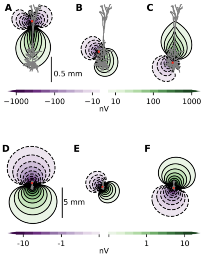
Figure 3.2: Simulation of extracellular potential showing distinct dipole pattern. The figure belongs to work carried out by Torbjørn Ness and Gaute Einevoll.
