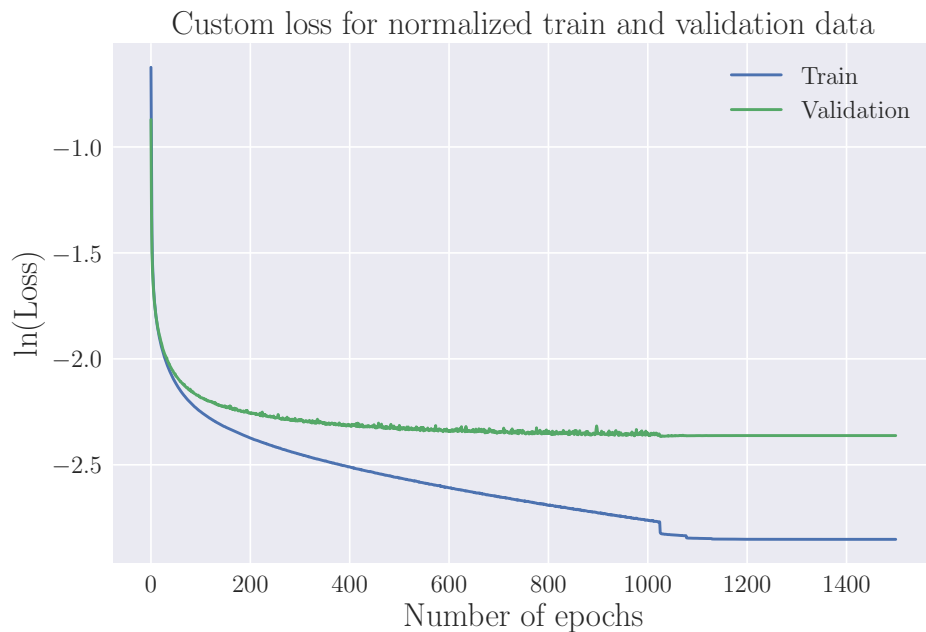
Figure 10.4: Training and validation loss as functions of epochs for the extended FCNN model, which predicts both location and magnitude parameters. The analysis is based on simulated data comprising 50,000 samples and spans a training duration of 1500 epochs.
