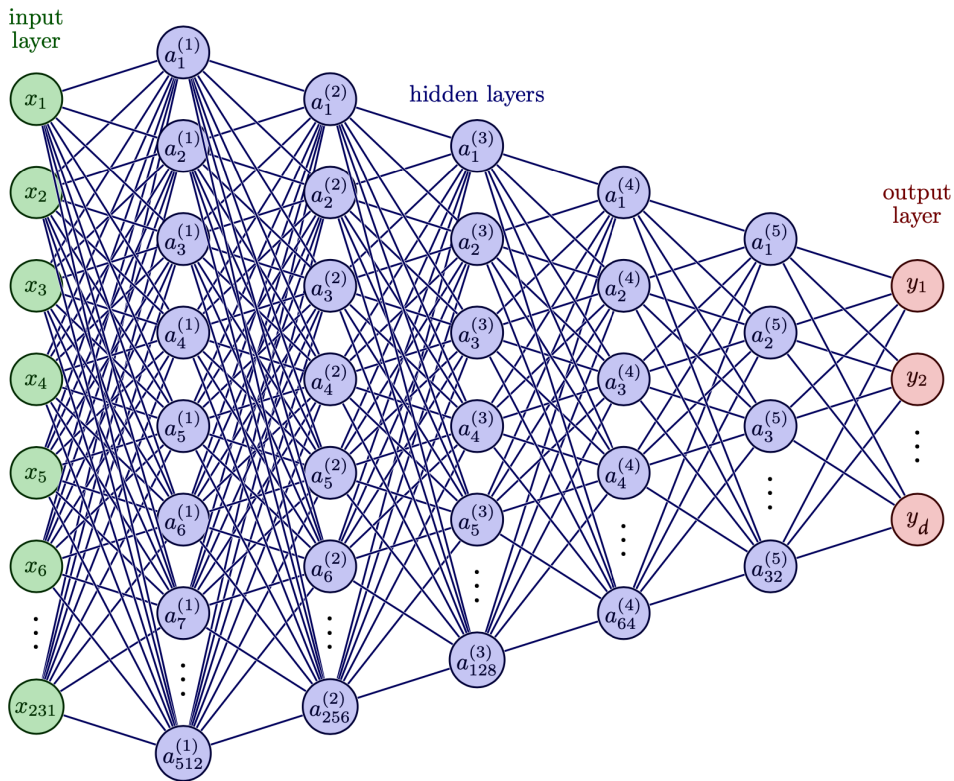
Figure 10.2: Architecture of the Extended Feed-Forward Neural Network. The input layer comprises 231 electrode recording input values, and the network outputs predicted d target values depending on the specific problem to solve. The FCNN consists of five hidden layers.
