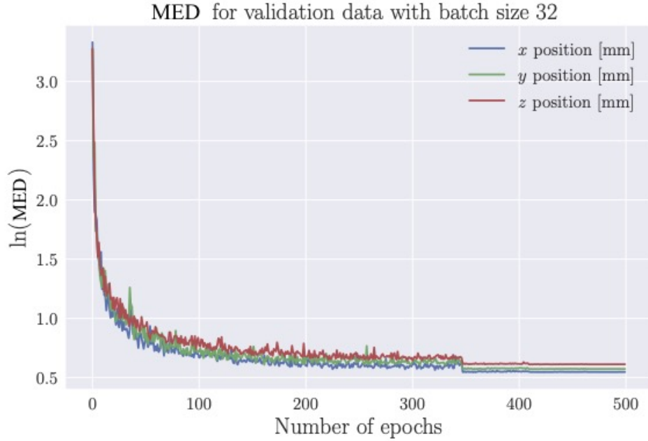
Figure 7.3: Validation MED loss for the separate target values; the x -, y -, z -coordinate.
