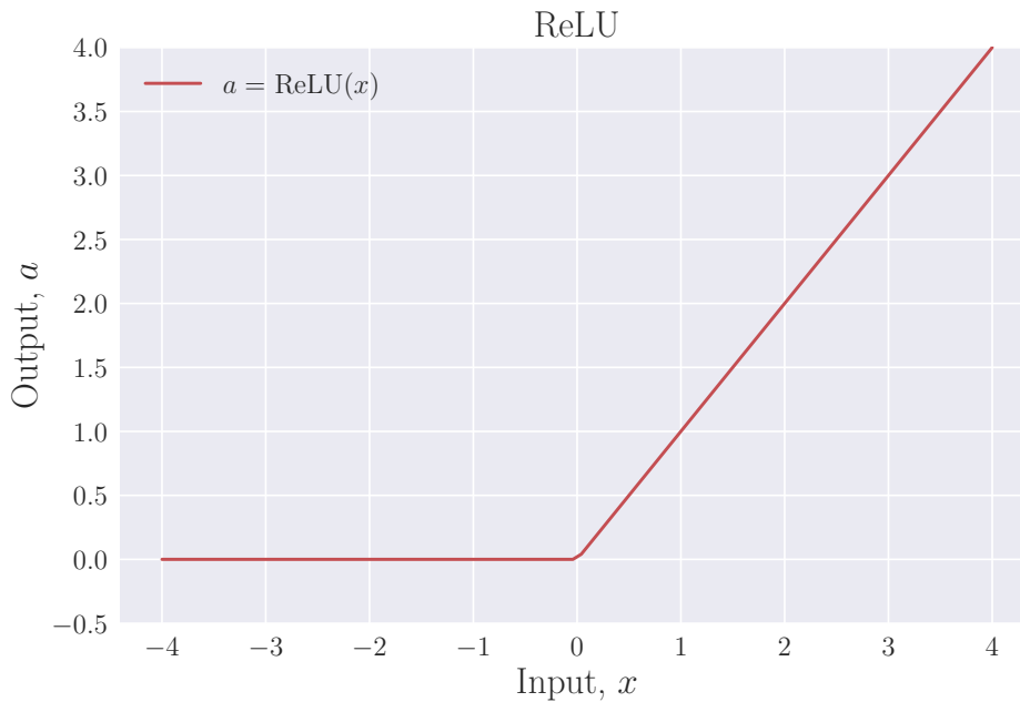
Figure 5.2: Rectified Linear Unit (ReLU) Activation Function: preserves positive input values x unchanged and enforces a transformation of negative input values to zero.
