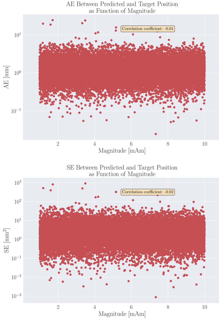
Figure 10.6: Scatter plot of Absolute Error and Squared Error computed between predicted and target coordinate values, as function of the magnitude of the dipole strengths.
