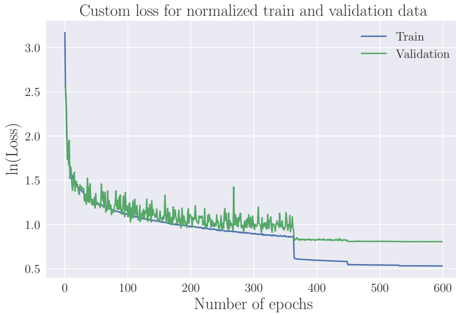
Figure 8.4: Training- and validation MED loss for the convolutional neural network with 50,000 samples and tanh as activation function.
