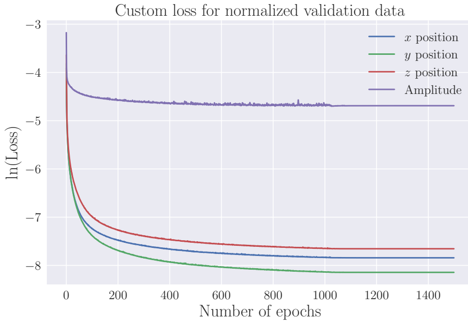
Figure 10.5: Validation loss as a function of epoch for each target value, including the x -, y -, and z -coordinates of the dipole, as well as the magnitude of the dipole signal.
