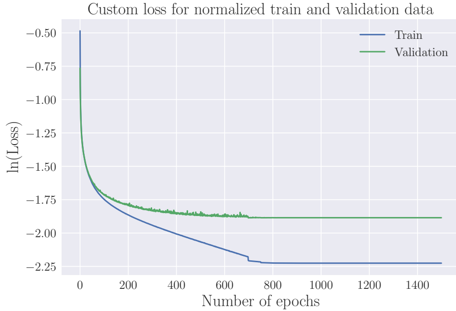
Figure 10.9: Training and validation custom loss trends as functions of epochs for the FCNN model, which predicts the center, magnitude, and radius of dipole populations. The analysis is based on simulated data comprising 50,000 samples and spans a training duration of 1500 epochs.
