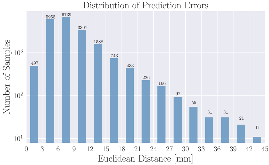
Figure 9.3: Histogram illustrating the Euclidean Distance for predicted dipole locations, organized into bins of width 3 mm. The ED thresholds are organized into bins of width 3 mm. Each bin holds the number of samples with prediction errors that falls within the given interval.
