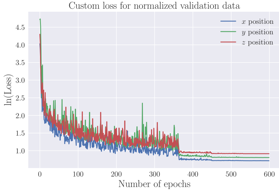
Figure 8.5: Training- and validation MED loss for the convolutional neural network with 50,000 samples and tanh as activation function.
