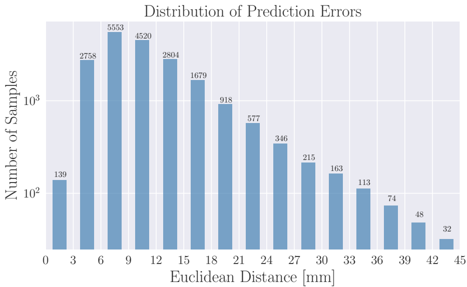
Figure 9.6: Histogram illustrating the Euclidean Distance for predicted dipole locations, organized into bins of width 3 mm.
