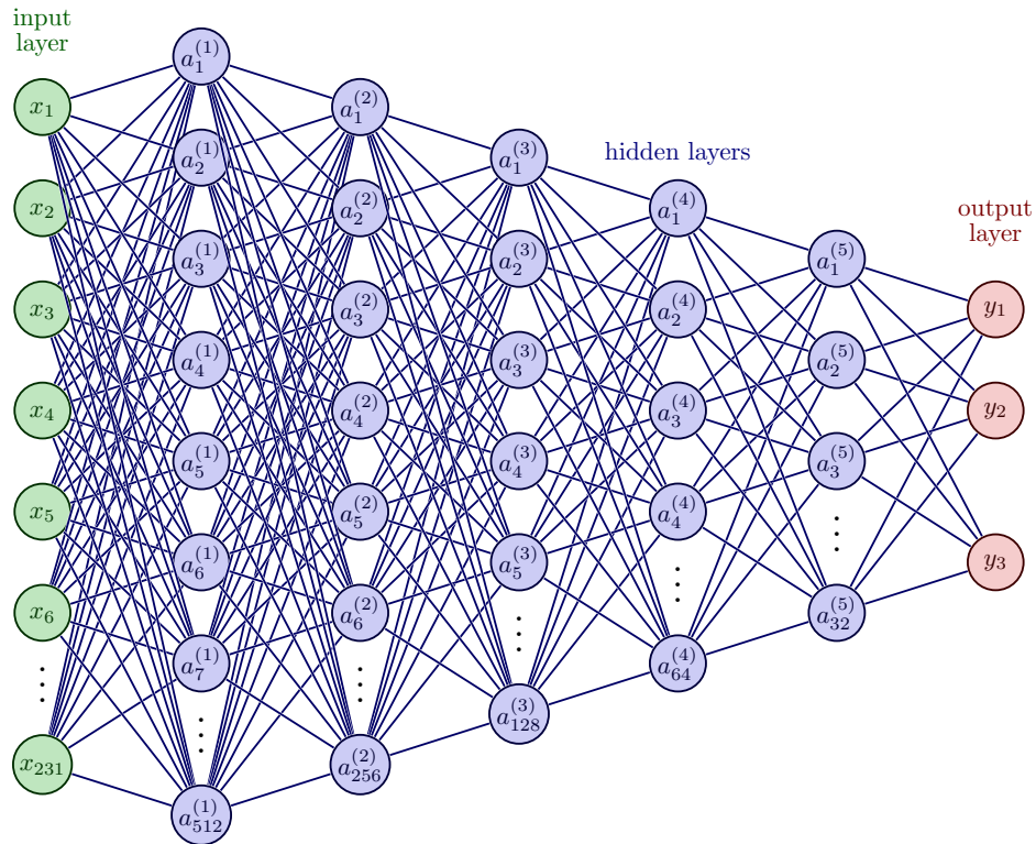
Figure 5.1: Architecture of the fully connected Feed-Forward Neural Network. The input layer comprises 231 electrode recording input values, and the network outputs predicted x -, y -, and z -coordinates of the dipole generating the EEG signal. The FCNN consists of five hidden layers. The visualization has been made with Latex, with code adapted from Neural Networks in TikZ with attribution to Izaak Neutelings and is licensed under the Creative Commons Attribution-ShareAlike 4.0 International License [27].
