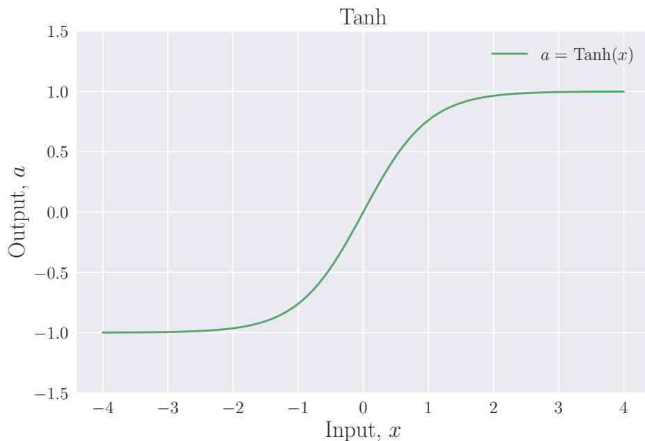
Figure 5.3: Hyperbolic tangent activation function: maps the input value x into a continuous range between -1 and 1 .
