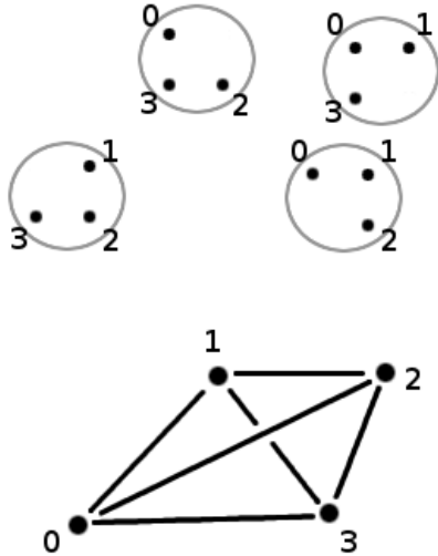
Figure 3.2.7: The symmetric container \partial(\mathbb{Z}_4 \triangleright C_4) .
