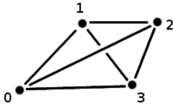
Figure 3.2.7: The symmetric container \partial(\mathbb{Z}_4 \triangleright C_4) .
