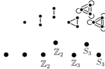
Figure 3.6.9: The first components of a possible solution to the differential \partial F \simeq F \times F , given \llbracket F \rrbracket(0) = 1 .
