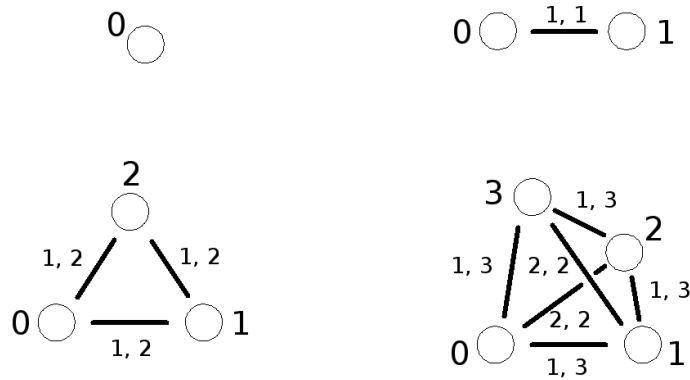
Figure A.1: The first four components of B(\mathbb{Z}_*, C) . Each line represents a pair of isomorphisms going opposite in directions. Identity morphisms excluded.
