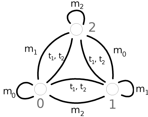
Figure A.2: The translation groupoid of S_3 acting on Fin(3) . The elements of S_3 are the identity (not shown), the translations t_1 and t_2 and the reflections m_0 , m_1 and m_2 .
