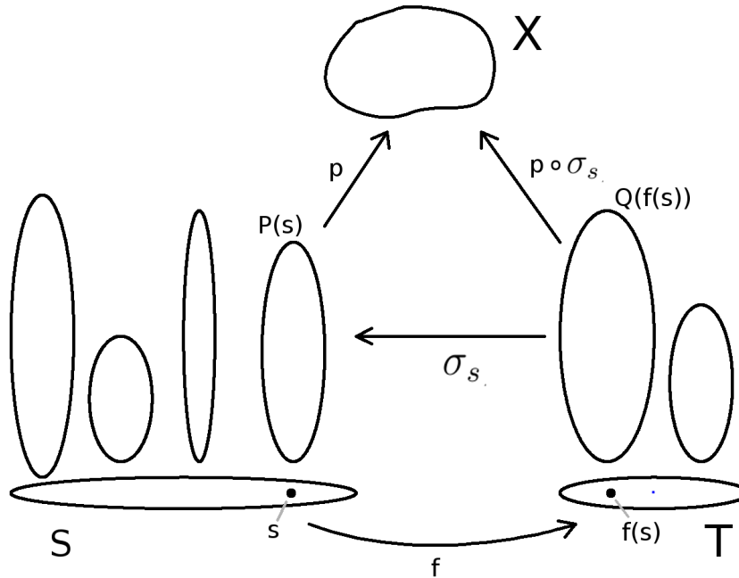
Figure 1.2.2: A figure illustrating how a container morphism (f, \sigma) lets you translate (s, p) into (f(s), p \circ \sigma_s) . Here we picture the sets of positions as stalks above S and T .
