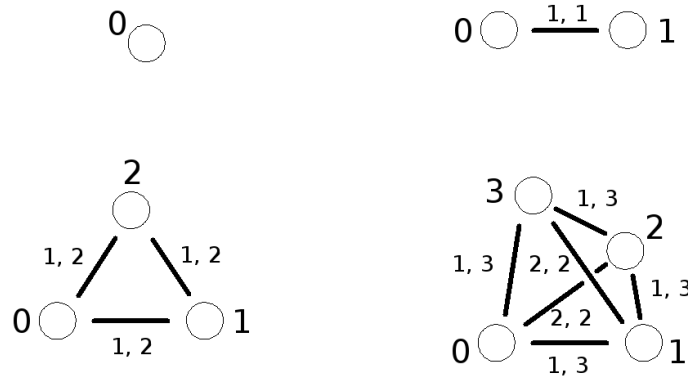
Figure 3.5.8: The first four components of B(\mathbb{Z}_*, C) , the groupoid of shapes in \partial(\mathbb{Z}_* \triangleright C) . (Identity morphisms not included.)
