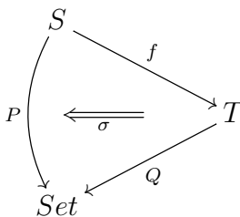
Figure 1.2.1: A diagram of a container morphism (f, \sigma) between the containers S \triangleright P and T \triangleright Q
