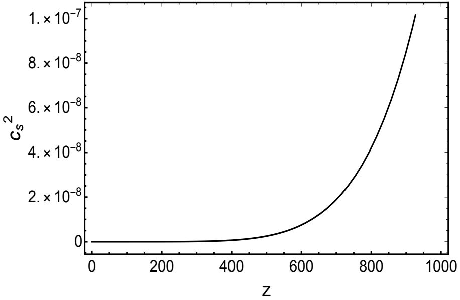
Fig. 1. Plot for c_s^2 vs z . As can be seen, the sound speed is very small compared to the speed of light ( c = 1 in this case) at all times.
