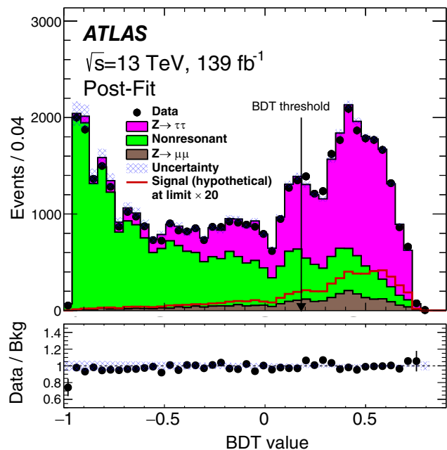
FIG. 1. Distributions of BDT values for samples of simulated Z \rightarrow e\mu signal and background events (histograms), as well as data (points). The component labeled “nonresonant” includes all SM background processes except Z \rightarrow \tau\tau and Z \rightarrow \mu\mu . The normalizations for the Z \rightarrow \tau\tau , Z \rightarrow \mu\mu , and nonresonant background use the best-fit values in Table I. A hypothetical Z \rightarrow e\mu signal, whose branching fraction is set to 20 times the observed upper limit, is shown with a dark red solid line for illustration purposes. The uncertainty band for the MC histogram distribution includes both the systematic and statistical uncertainty. An arrow is added to show the analysis selection requirement for the BDT, corresponding to a value of 0.18.
