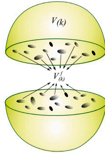
Fig. 2. Integrated volume of voids V_{(k)}^f within the peridynamic particle volume V_{(k)} .
