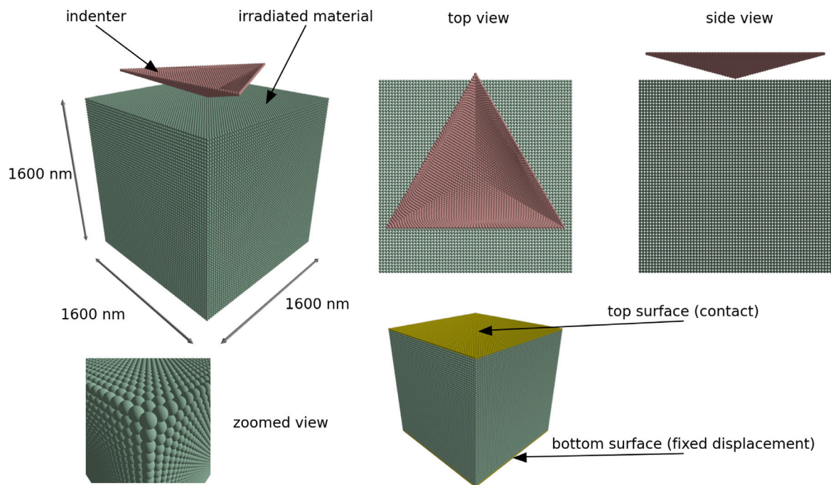
Fig. 13. Discretized peridynamics model of indentation test.
