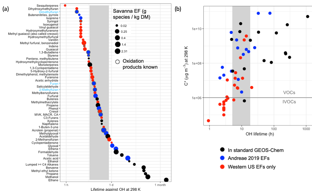
Figure 1. (a) NMOGs emitted from fires, shown in descending order of chemical lifetime due to oxidation by OH (at 298 K with an assumed concentration of 1 \times 10^6 \text{ molec. cm}^{-3} ). Only the species responsible for 95 % of OHR from fires are shown (following Coggon et al., 2019). Fire NMOGs included in the standard GEOS-Chem model are in black, species for which fire emissions are not included in the standard GEOS-Chem model but for which emissions factors are available in Andreae (2019) are in blue, and species that are only available for western US fuel types from Koss et al. (2018) are in red. The y-axis tick marks are in black for fire NMOGs added to GEOS-Chem in this study and in blue (with blue labels) when both the fire NMOG and its oxidation chemistry were added. The points are sized by their relative savanna and grassland (labeled “savanna”) emission factor in gram species per kilogram DM burned. The grey vertical box represents an approximate physical lifetime against transport out of a nested 0.5^\circ \times 0.625^\circ grid box ( \sim 5 \text{ h} ) and a 2^\circ \times 2.5^\circ grid box ( \sim 20 \text{ h} ). CA stands for crotonaldehyde. (b) Plot of volatility ( C^* ) against OH lifetime for the species shown in (a) using the same color conventions. The horizontal line separates VOCs from IVOCs based on their C^* .
