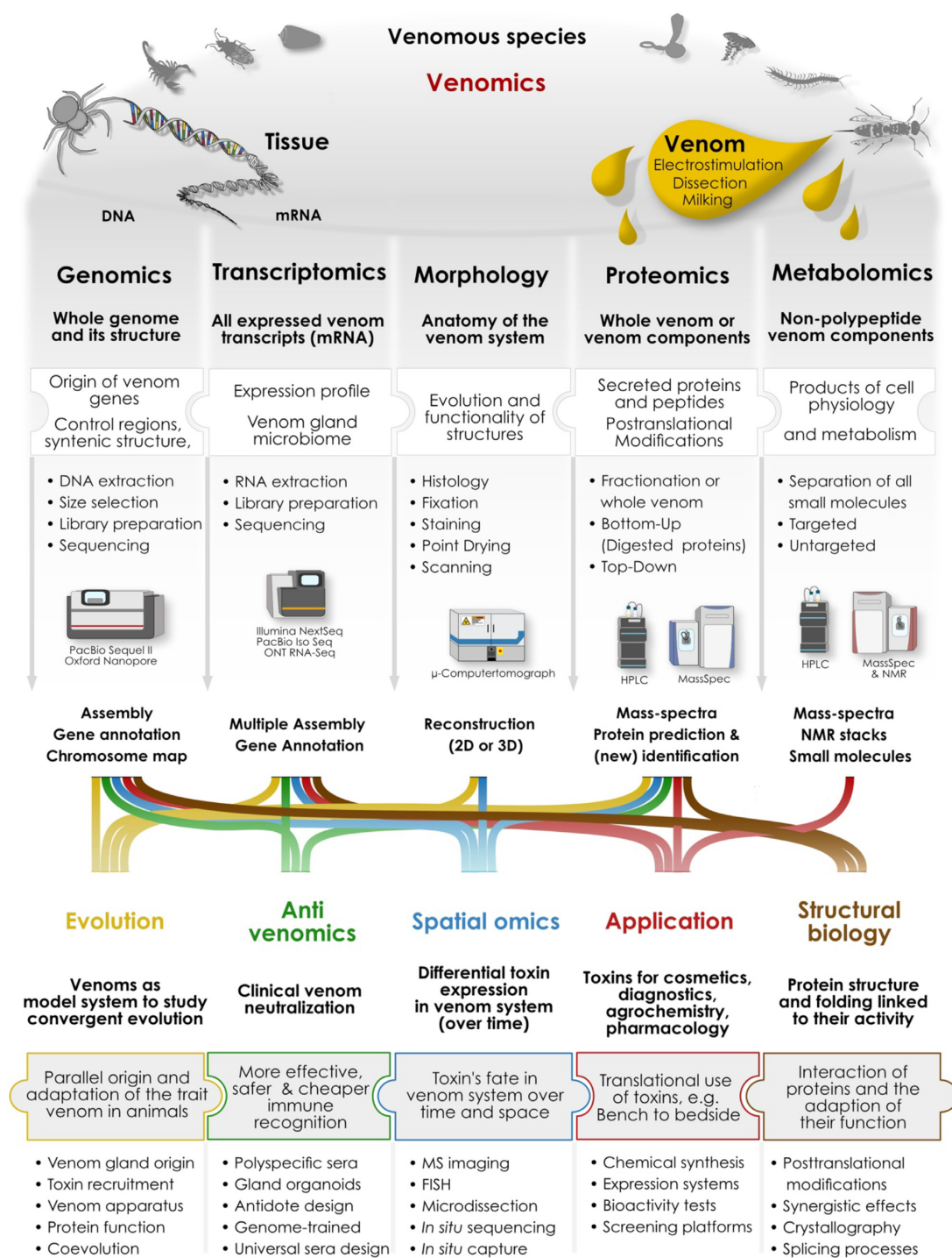
Figure 3: The major interdisciplinary research areas in venomomics. The basic, interlinked, modern research fields in venomomics are shown in the first row, and linked through simplified workflows with the final output(s). The main applied and evolutionary questions addressed are shown in the bottom, and integrated in the relevant topics. The flow diagrams that connect most research areas with each other illustrate the highly integrative nature of modern venomomics. FISH: fluorescence in situ hybridization.
