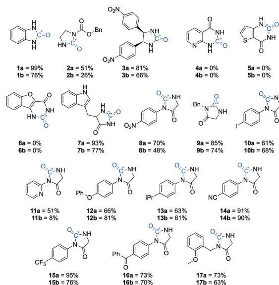
Fig. 1 Results for the direct incorporation of ^*\text{CO}_2 ; (a) NMR yield from ^{\text{nat}}\text{CO}_2 and (b) isolated yield of the carbon-13-labelled compound.
