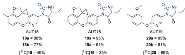
Fig. 2 Isotopic labelling and radiolabelling of drug candidates using ^{13}\text{C} (a) NMR yield (b) isolated yield with ^{13}\text{C} .
