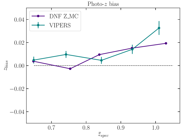
Figure 3. z_{bias} as a function of \bar{z}_{spec} , for the two z_{spec} estimates (VIPERS and Z MC ). z_{bias} is defined as the average difference between Z MEAN and the given redshift. After finding a good agreement between independent estimates, we assume the VIPERS validation as our default choice. Errors only apply to the VIPERS sample, and they are estimated as the standard deviation from realizations (see Section 5.2).
