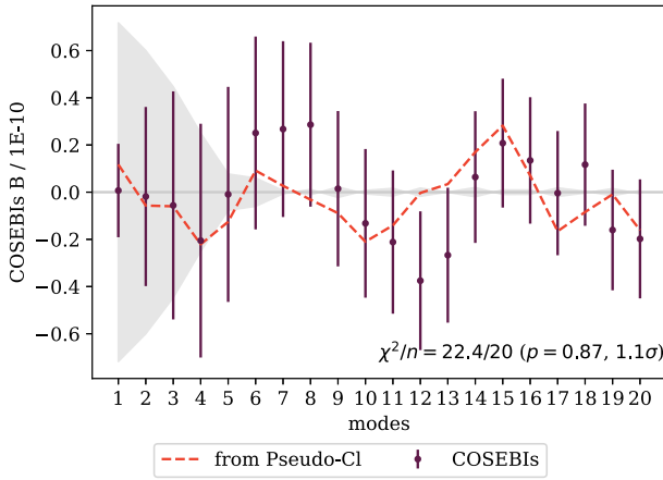
Figure 18. COSEBIs B modes from the DES Y3 shape catalogue are shown as data points with uncertainties given by a noise-only analytical covariance matrix. The dashed line shows the pseudo- C_\ell shown in Fig. 17 converted to COSEBIs B mode as described in the text. Note that the COSEBIs are always discrete measurements for individual modes, but the dashed line is connected for clarity. As an order of magnitude comparison, we show as a grey shaded region 10 per cent of the expected COSEBIs E mode of the weakest cosmic shear signal (the lowest redshift tomographic bin).
