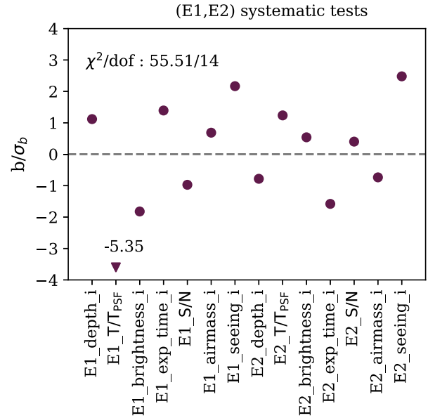
Figure 19. Best-fitting values for the coefficient of the relation \langle e_i \rangle = b \text{ syst} + c with \text{syst} a given systematic map. The values of the slopes are shown for different tomographic bins, and the uncertainties are estimated through lognormal mocks. We also tested using uncertainties estimated by jackknife resampling, with no sensible difference. The reported \chi^2 takes into account correlations among different systematic maps.
