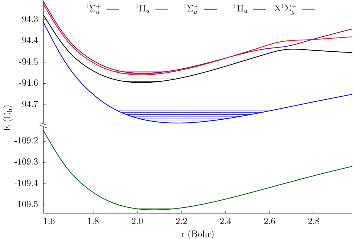
FIG. 8: Potential energy surfaces of ground and excited states and vibrational levels calculated with CC3/d-aug-cc-pCVQZ.
