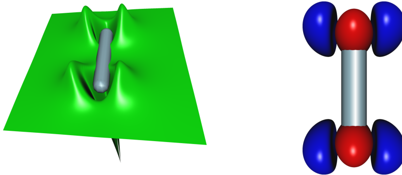
FIG. 9: Difference in electron density between the ground state and the lowest energy {}^1\Pi_u core-excited state in the plane and as isosurfaces. Red indicates reduced density and blue increased. Isovalue: 0.01
