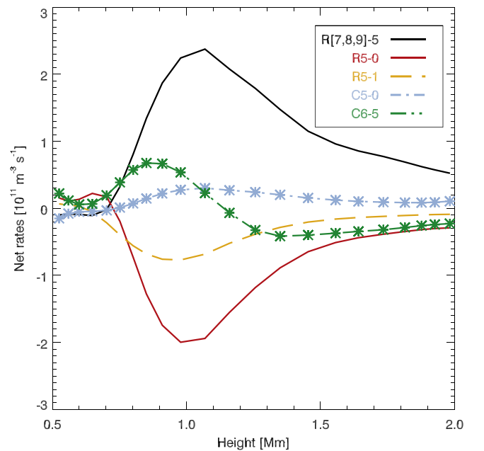
Figure 3. Net rates to 2p^3 3s^5 S_2 , (level 5 in the O I model atom (Figure 1)). Positive values denote a net rate coming into the level, negative values a rate going out of the level. Letters R and C in the label stands for radiative net rate and collisional net rate, respectively. The collisional net rates are also overlaid with star symbols. The dominant channel into the 2p^3 3s^5 S_2 level is from the three levels in the 2p^3 3p^5 P term, (levels 7, 8, 9, solid black). The secondary channel is through collisions from the 2p^3 3s^3 S_1^o term (level 6, green dot-dashed with stars). The 2p^3 3s^5 S_2 level is depopulated by the emission lines at 135.56 nm (solid red) and 135.85 nm (dashed yellow). There is also a collisional rate, C5-0, corresponding to the 135.56 nm line (dot-dashed blue with stars).
