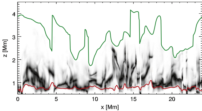
Figure 8. Contribution function to the intensity of the O I line core along a cut through the atmospheric model at X = 12 Mm together with the \tau = 1 height of the line core (red solid line) and temperature contour at 30 kK (green). The contribution function has been individually scaled for each column for increased visibility. Note that the z -axis has been stretched.
