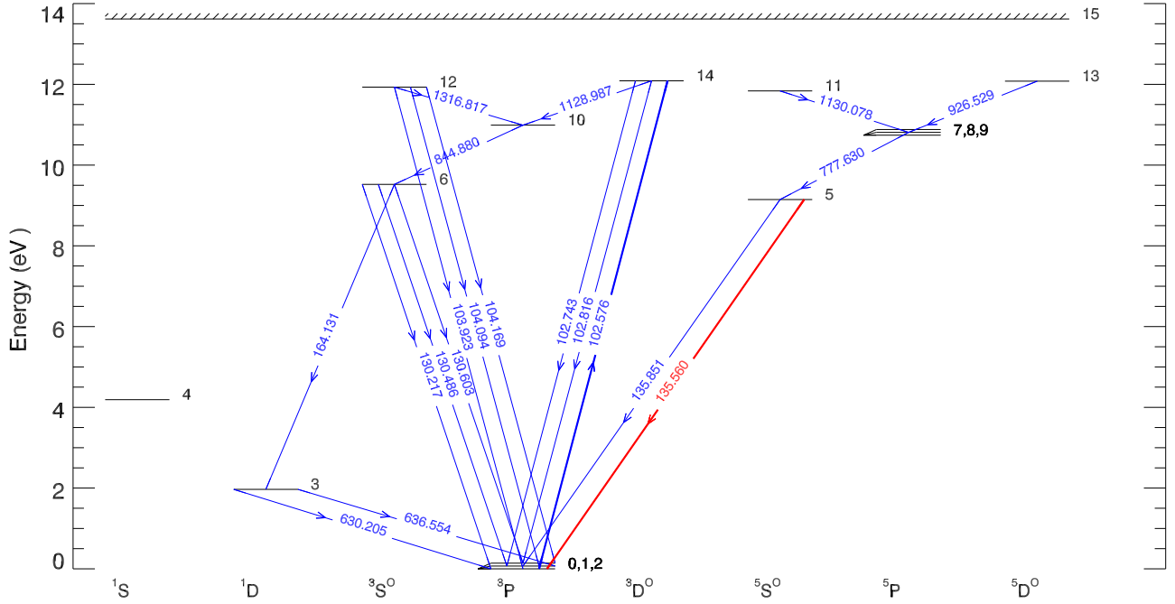
Figure 1. Term diagram of the 16 level O I quintessential model atom used in this study. The energy and designation of each numbered level is listed in Table 1. The arrows show the direction of the net rates for each transition in the chromosphere. Vacuum wavelengths are shown in nm. The energies of the levels of the terms 2p^4\ ^3P (levels 0, 1, 2) and 2p^3\ 3p\ ^5P (levels 7, 8, 9) are very close to each other and the energy differences within these terms are exaggerated in this diagram. The transitions to or from levels 7, 8 and 9 are represented by the transition to and from level 8 ( 2p^3\ 3p\ ^5P_1 ) only. The O I 135.56 nm line that is the topic of this paper is shown in thick red, the 102.576 nm line that is pumped by the hydrogen Ly \beta line is in thick blue.
