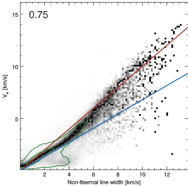
Figure 12. PDF of V_w (Equation (14)) as a function of the non-thermal broadening, W_{\text{nth}} , of the line profile (Equation (13)). Each column is scaled to maximum contrast to increase visibility. The green contours encompass 50% and 90% of all points. The Pearson linear correlation coefficient is given in the upper left corner. The diagonal red straight line denotes y = x , which is the expected relation for a Gaussian velocity distribution; the blue straight line denotes y = 0.68 x , which is the expected relation for a flat velocity distribution.
