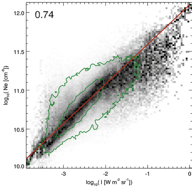
Figure 10. PDF of the logarithm of the contribution function weighted electron density as a function of the logarithm of the O I total line intensity. Each column is scaled to maximum contrast to increase visibility. The green contours encompass 50% and 90% of all points. The Pearson linear correlation coefficient is given in the upper left corner. The red line denotes the line \log_{10}N_e = 0.51 \log_{10}I + 12.10 , which is equivalent to I \sim N_e^{1.97} . For more details, see the discussion in Section 5.3.
