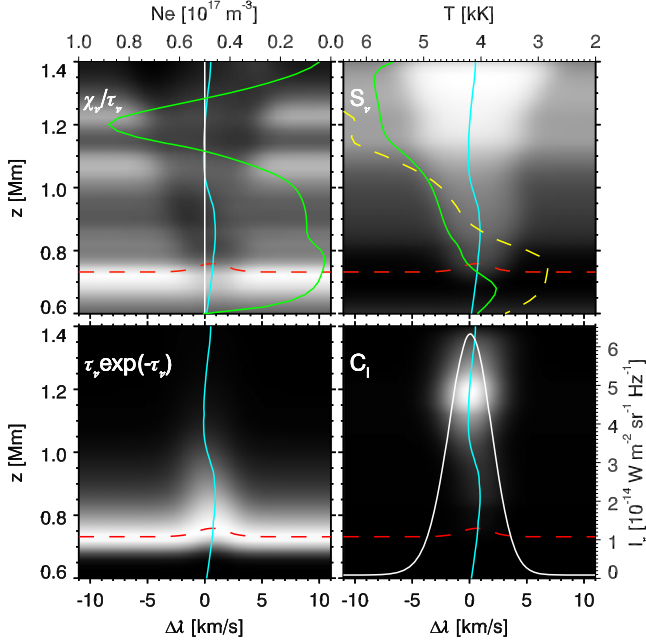
Figure 5. Intensity formation for the O I 135.56 nm line in a column of the 3D atmosphere characterized by moderate velocities. The label in the top-left corner of each panel gives the quantity shown as a gray-scale image as function of wavelength (given as Doppler shift from the rest frequency, positive means redshift) and height z . The \tau = 1 height is given as a red dashed line and the vertical velocity as a blue solid line in all four panels with a white straight line denoting the rest frequency in the upper left panel. The green solid line in the upper left panel gives the electron density with a scale at the top. In the upper right panel we show the temperature as a yellow dashed line and the source function at a frequency given by the velocity profile as a green line, both with the scale given at the top. In the lower right panel we show the full contribution function (the product of the terms shown as gray-scale images in the other three panels) together with the emergent intensity profile with a scale to the right.
