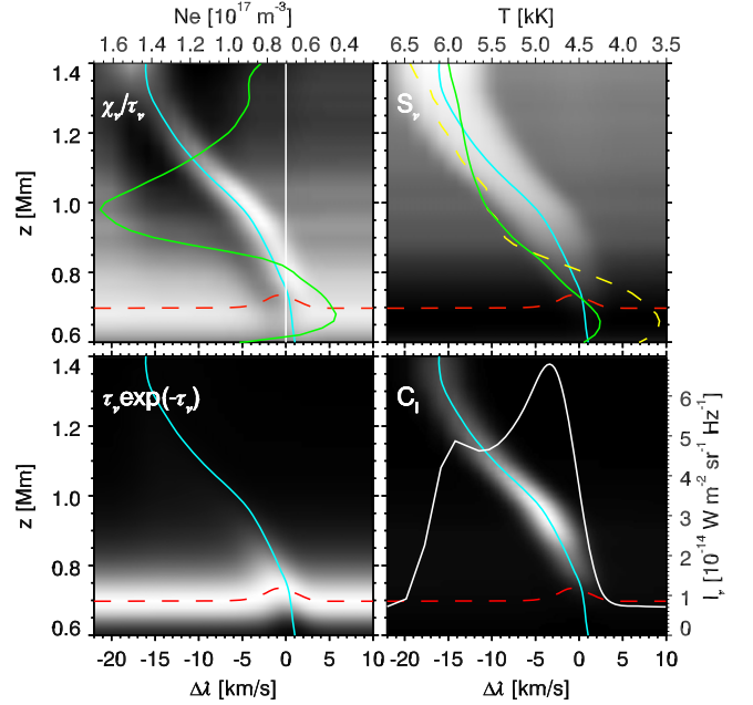
Figure 6. As for Figure 5, but for a column with a large velocity amplitude through the atmosphere ( \sim 15 \text{ km s}^{-1} ). The line profile is highly asymmetric and the line is broadened by the velocity range within the O I line forming region (0.7–1.4 Mm in this case). Note the expanded wavelength scale compared with Figure 5.
