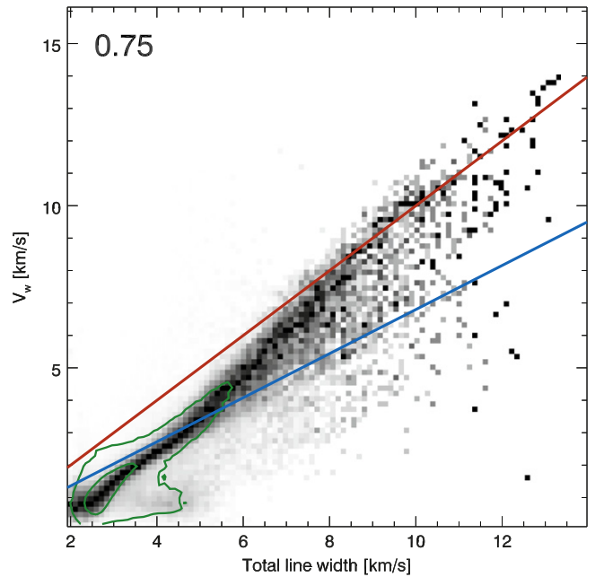
Figure 11. PDF of V_w (Equation (14)) as a function of the total broadening, W_{\text{total}} (Equation (11)). The green contours encompass 50% and 90% of all points. The Pearson linear correlation coefficient is given in the upper left corner. The diagonal red straight line denotes y = x , which is the expected relation for a Gaussian velocity distribution; the blue straight line denotes y = 0.68x , which is the expected relation for a flat velocity distribution.
